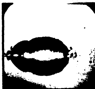
Figure 28: Nonspherical Sequence in Water
