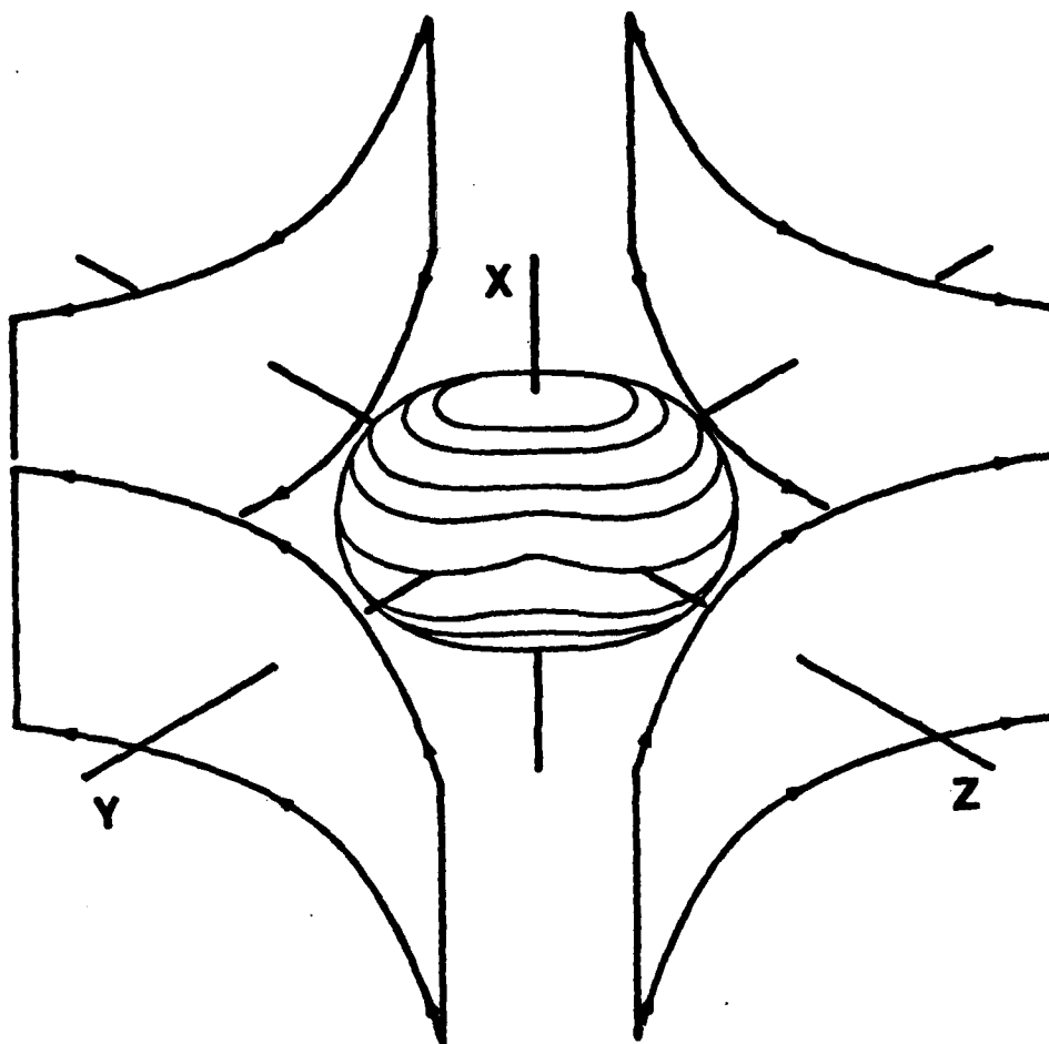
Figure 8. Representative Bubble Shape \eta_i and External Flow for Y_2(\theta, \phi) Stream surfaces are shown along with bubble shape.
