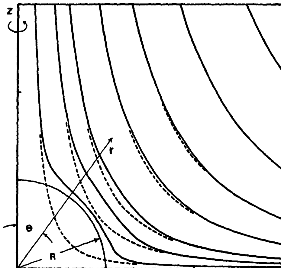
Figure 10. Alteration of Streamlines by Sphere for Y_2^0(\theta, \phi) without sphere \leftrightarrow pure extension with sphere \leftrightarrow v_1^{\infty}
