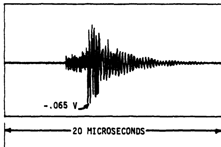
FIGURE V-5. WIRE DATA; RADIATED PULSE PARALLEL TO THE FUSELAGE; ONE SIDE OF THE INTERIOR WIRES GROUNDED
