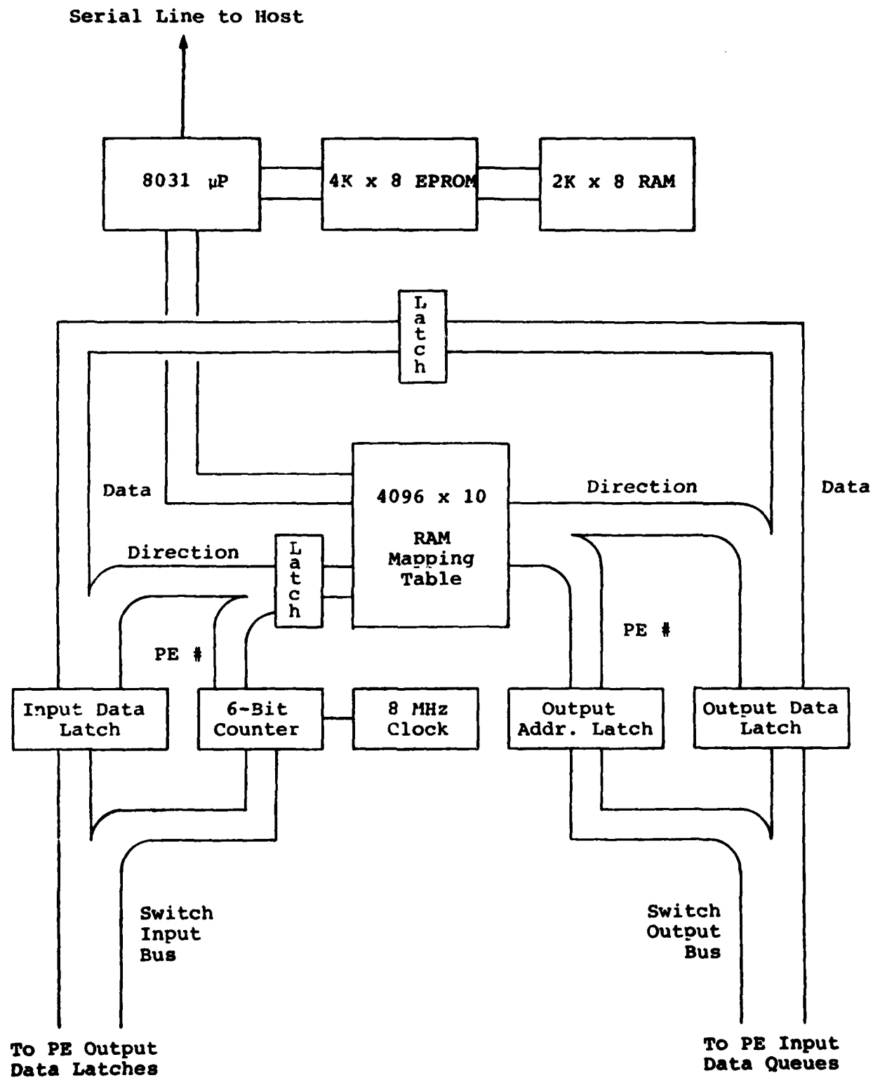
Figure 5. Switch Detail.
