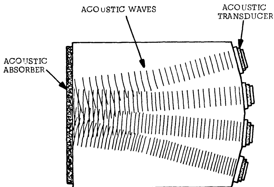
FIGURE 12. ALTERNATE ACOUSTO-OPTIC COMPONENT DESIGN.
