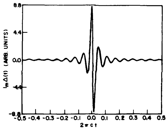
Figure 3. Real and Imaginary Parts of the Difference Function, \Delta(t) , Calculated From an Approximate \phi(t)
