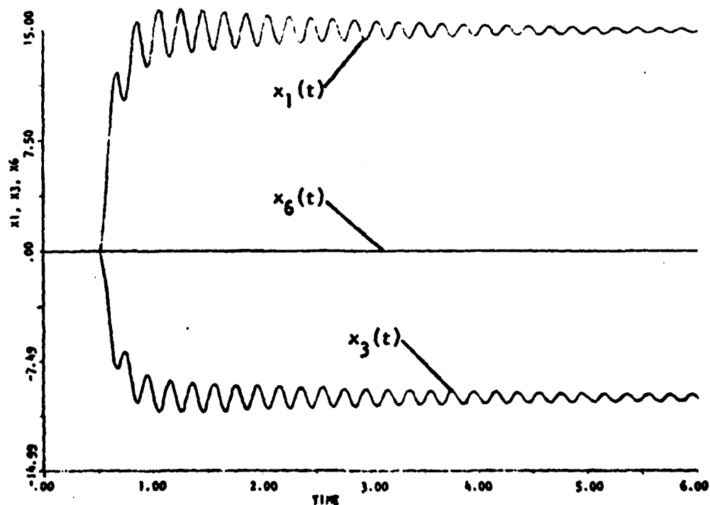
Figure 12. x_1(t) , x_3(t) , and x_6(t) , Example 3.
