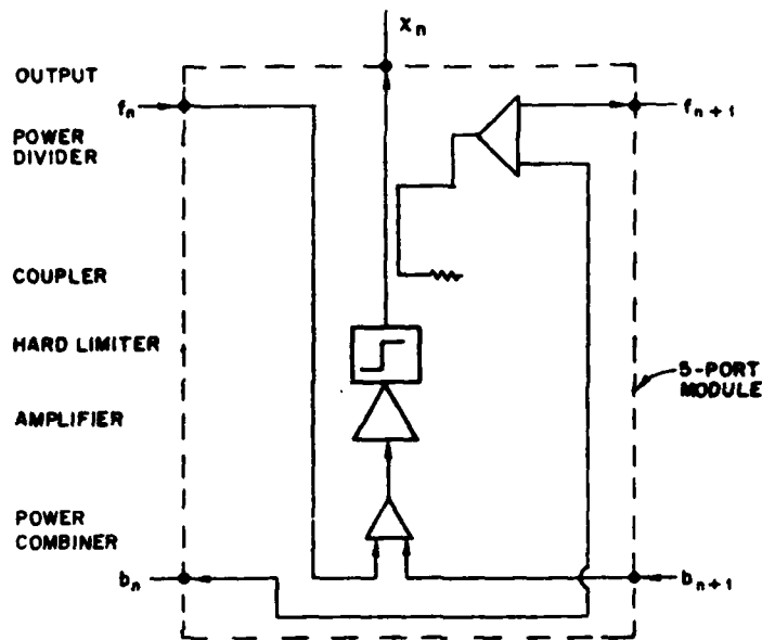
Fig. 3 — Amplifier/limiter module for coupled amplifier module feed
