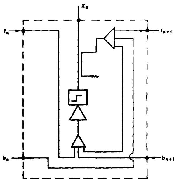
Fig. 12 — Amplifier/limiter module with self-coupling
