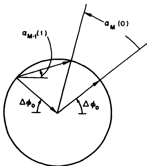
Fig. B3 — Phasor diagram derived from Eq. (B13), assuming F > 0 . The S = 0 phase distribution (cf. Fig. 5) evolves when angle \alpha_{M-1}(1) < \pi , i.e., for 0 < \alpha_M(0) < (\pi - 2\Delta\phi_0) .
