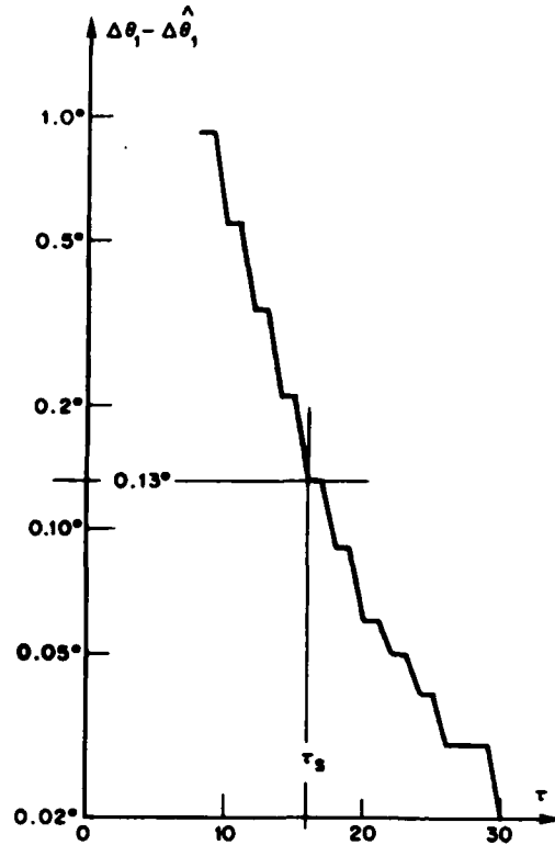
Fig. 9 — Values plotted are the difference between the exact value of \Delta\theta_1 (Fig. 8) and the approximate value \Delta\hat{\theta}_1 obtained from Eq. (35). Error incurred in using \Delta\hat{\theta}_1 is less than 0.13^\circ for \tau > \tau_s .
