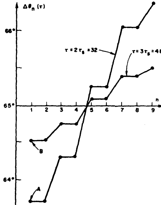
Fig. 7 — Phase distribution for an 8-module feed at two values of time ( \tau = 32 and \tau = 48 ). Assumed parameter values were (M, \Delta\phi_0, \alpha_M(0)) = (9, 60^\circ, 45^\circ) . In the infinite-time limit a uniform phase gradient is established, \Delta\theta_n(\infty) = \Delta\phi = 65^\circ .
