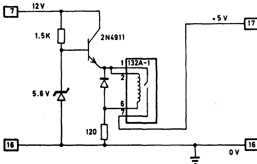
Fig 9 Voltage regulator
