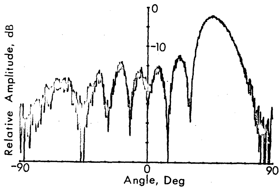
Figure 37. Beam scanned to 48^\circ ( \alpha = 135^\circ )
