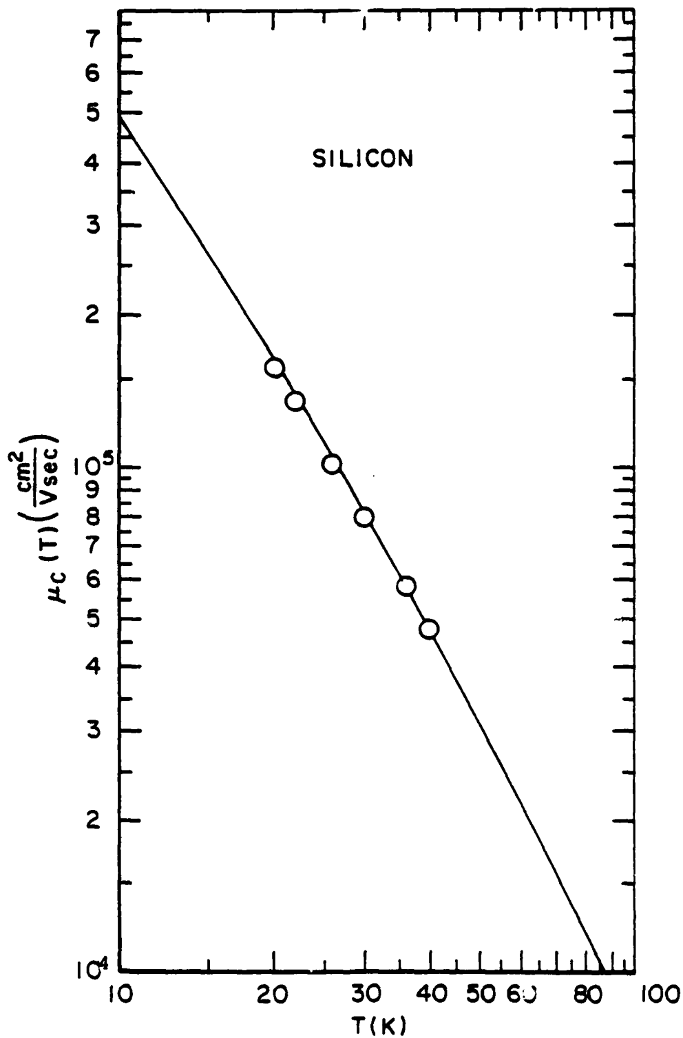
Fig. 27. Calculated conductivity mobil. \mu_c for silicon (solid line) and the experimer al data for sample 1202-H.
