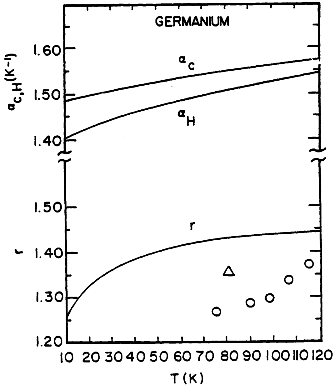
Fig. 10. Top scale: Calculated temperature exponents \alpha_c for the conductivity mobility, and \alpha_H for the Hall mobility (solid line).
