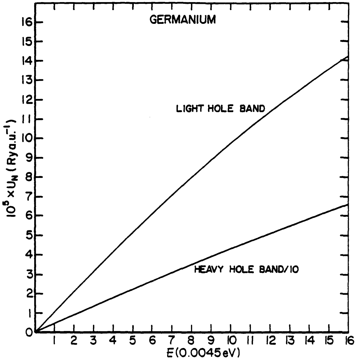
Fig. 5. Temperature independent part of the integrand in the numerator of Eq. (53a) for \mu_c , defined by Eq. (79).
