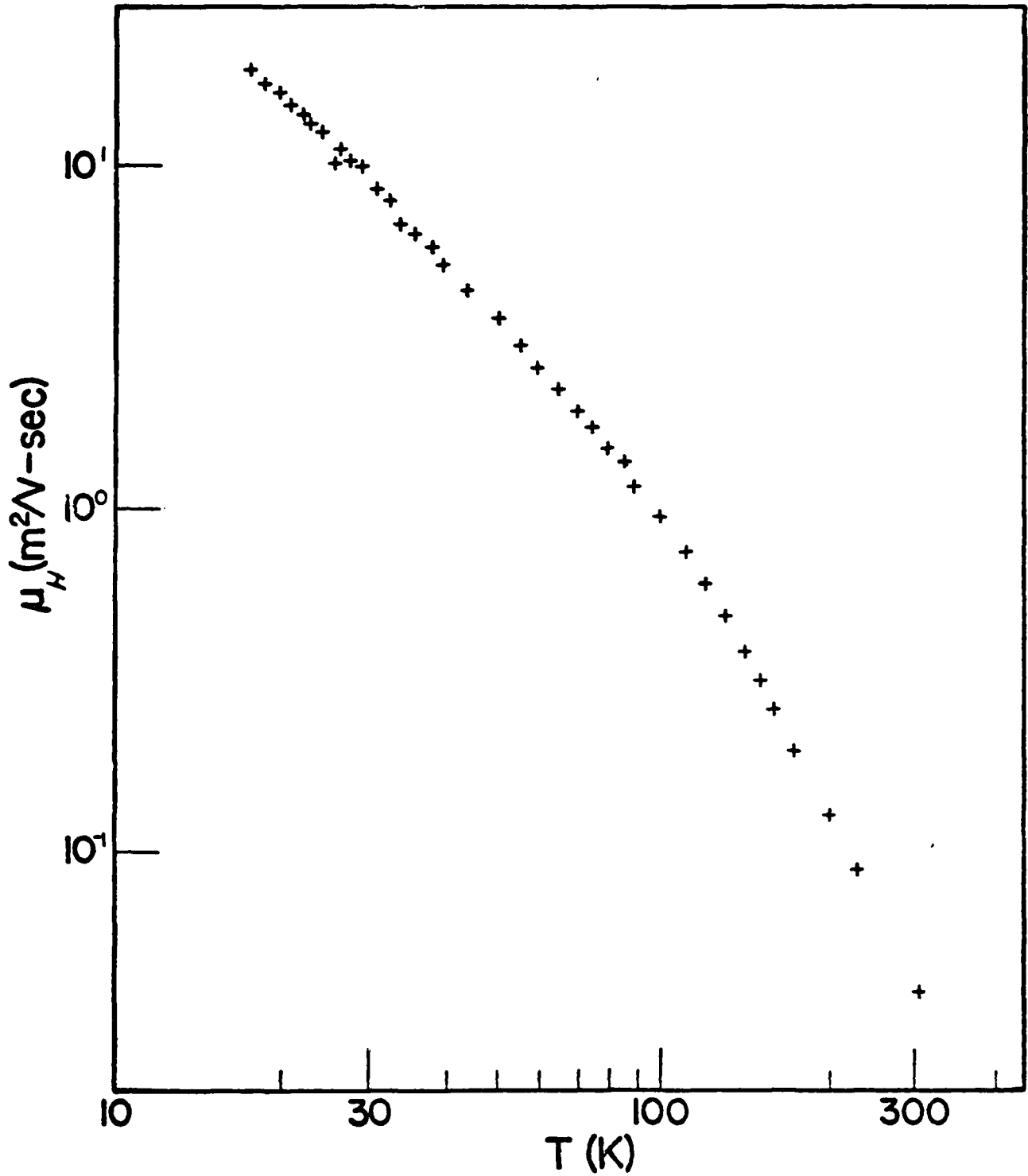
Fig. 15. 0.1T Hall mobility for sample 1202-H.
