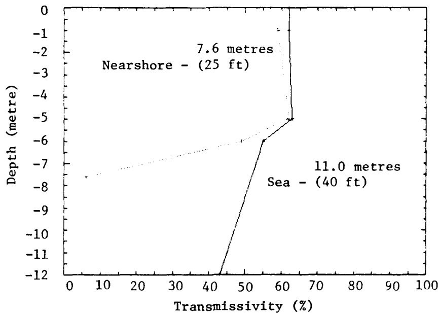
FIGURE 28. TRANSMISSIVITY ON 1 SEPTEMBER 1981
