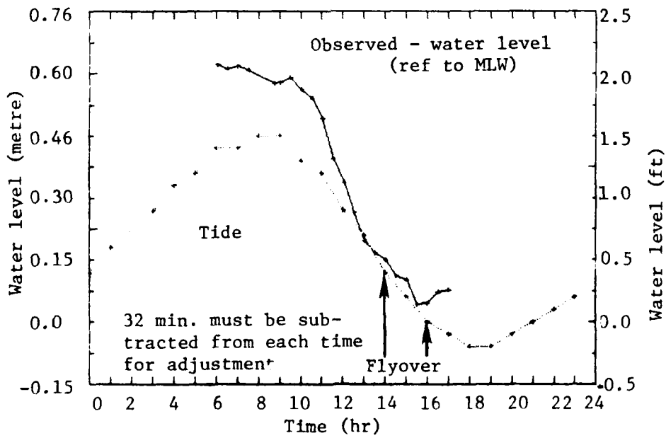
FIGURE 10. WATER LEVEL/TIDAL CURVE ON 27 AUGUST 1981
