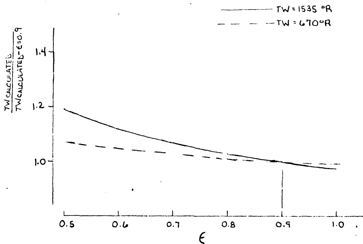
Figure 8. Emissivity-Temperature Sensitivity Curve
