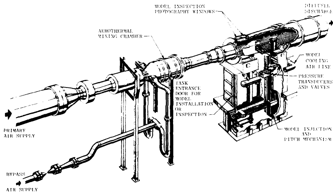
b. Perspective of tunnel test section area
