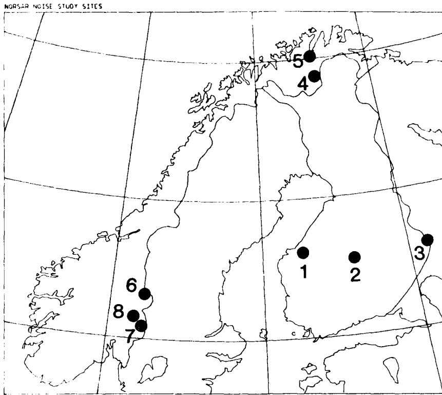
Fig. VI.7.1 Sites for the Fennoscandian noise survey 1981/82.
