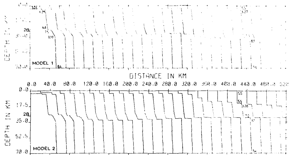
Fig. VI.6.8 Velocity-depth distributions for Models 1 and 2. The first order discontinuity in the crust after 340 km for Model 2 has not been observed and serves only to signify a decrease in the mean crustal velocity in that area.
