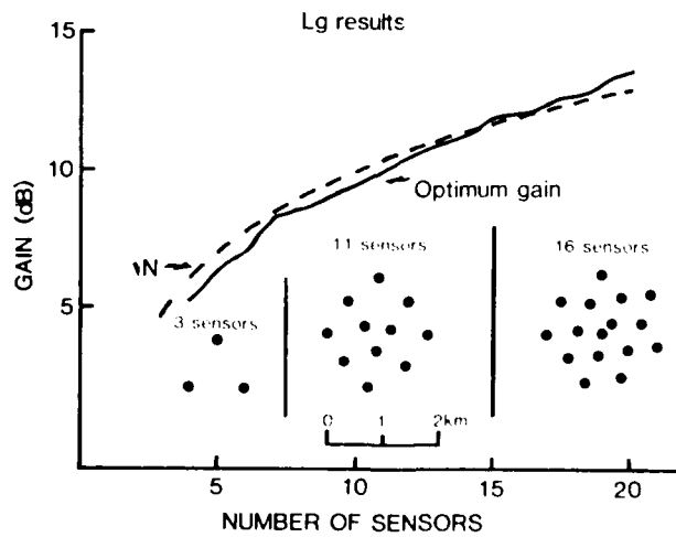
Fig. VI.3.6 Same as Fig. VI.3.5, but for the Lg phase.
