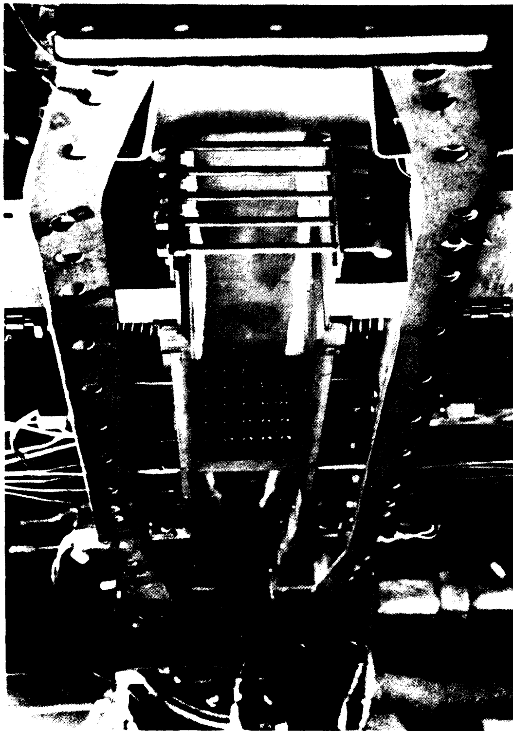
FIGURE 1. PHOTOGRAPH OF TEST COMBUSTOR
