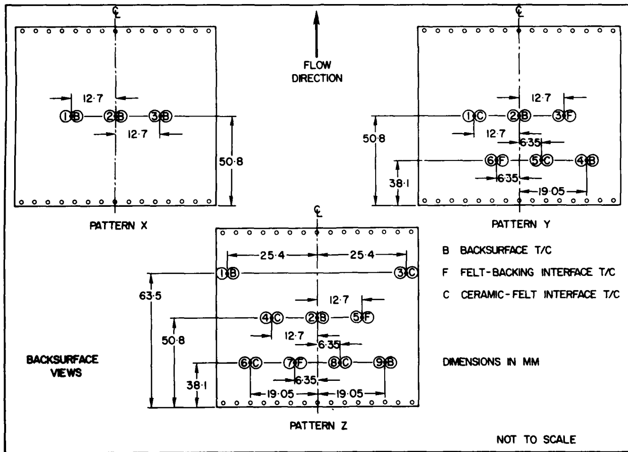
FIGURE 6. TEST PANEL INSTRUMENTATION LAYOUT
