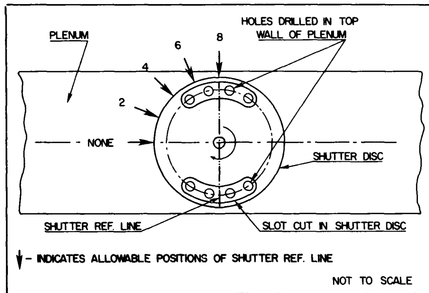
FIGURE 3. VARIABLE COOLING AIR MECHANISM
