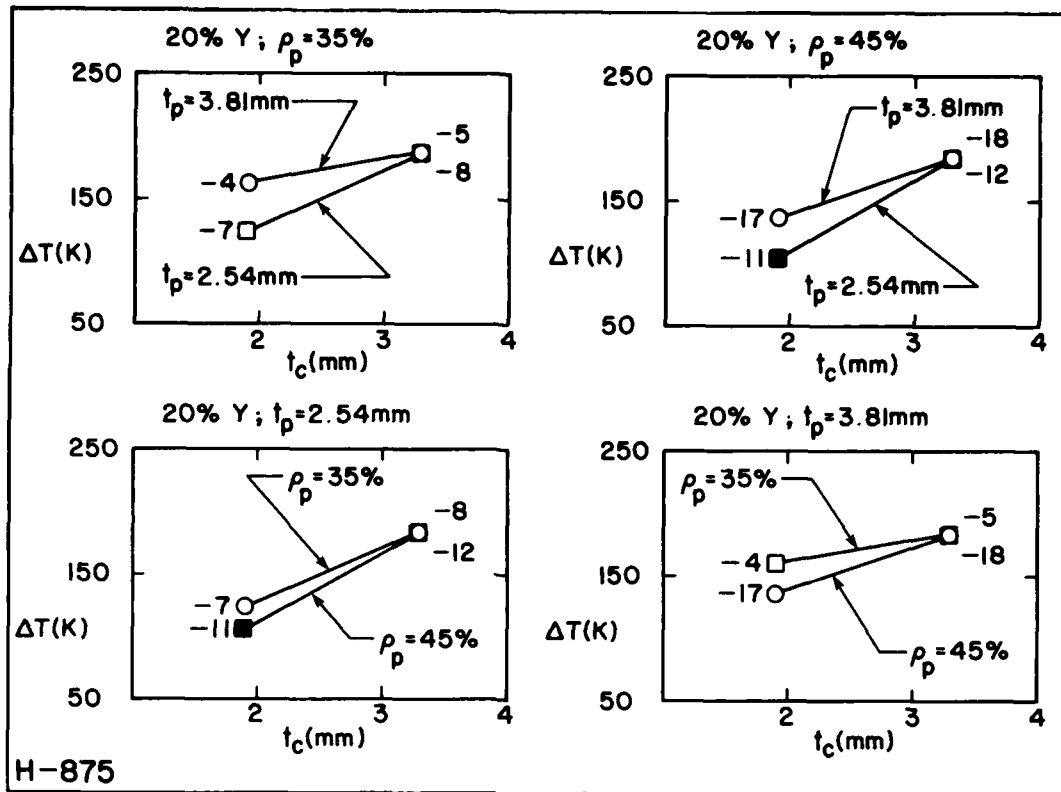
FIGURE 13. EFFECT OF CERAMIC THICKNESS ( t_c ) ON THE CERAMIC STRESS LEVEL ( \Delta T ) FOR THE H-875 PAD MATERIAL
