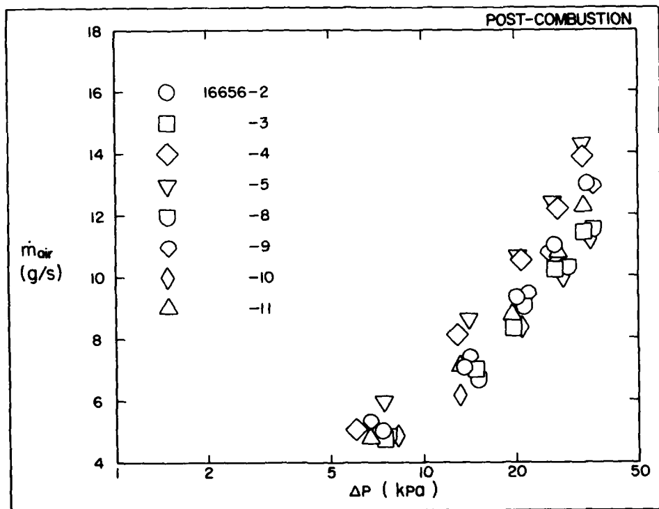
FIGURE 12. FLOW CHARACTERISTICS OF TRANSPIRATION COOLED PANELS
