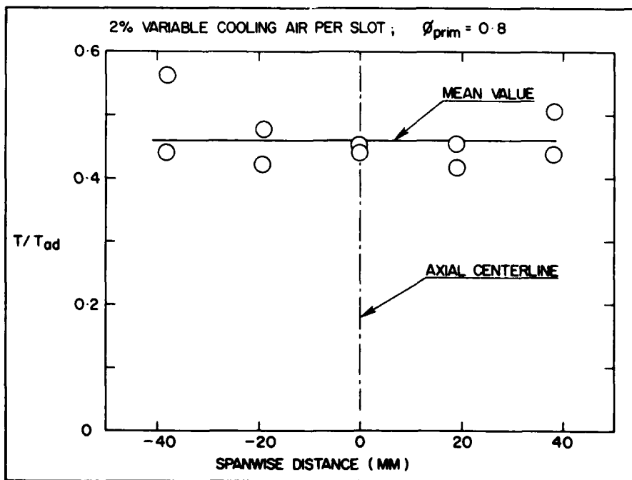
FIGURE 11. SPANWISE TEMPERATURE DISTRIBUTION
