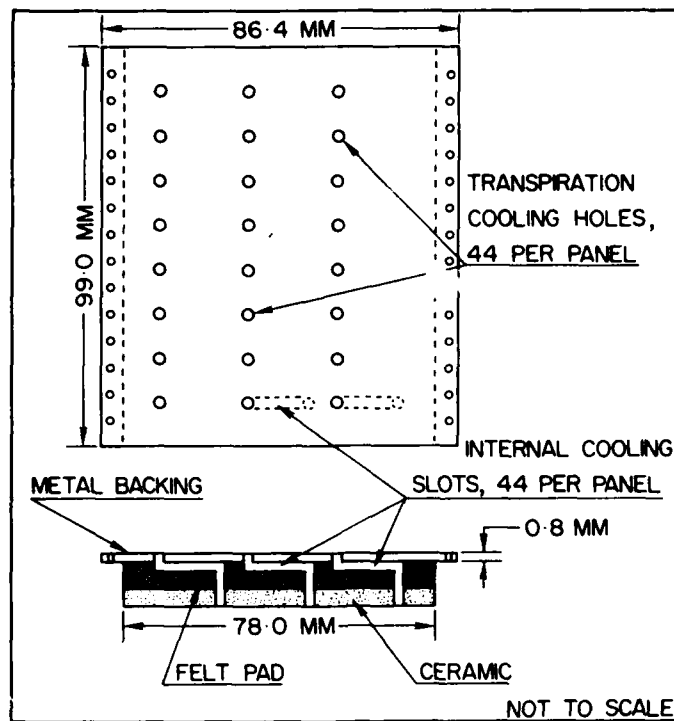
FIGURE 5. TEST PANEL DESIGN
