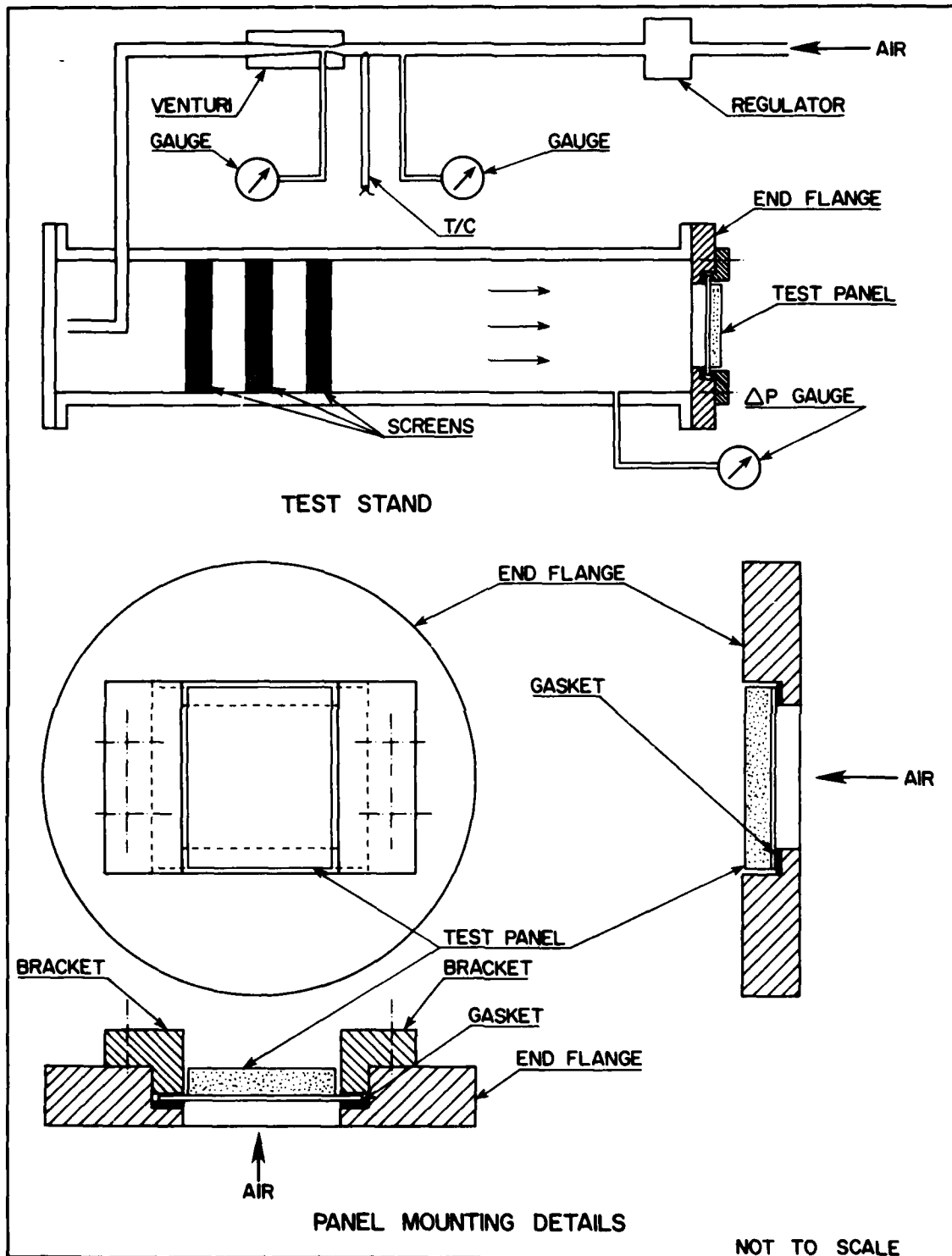
FIGURE 8. ATMOSPHERIC TEST STAND AND PANEL MOUNTING DETAILS
