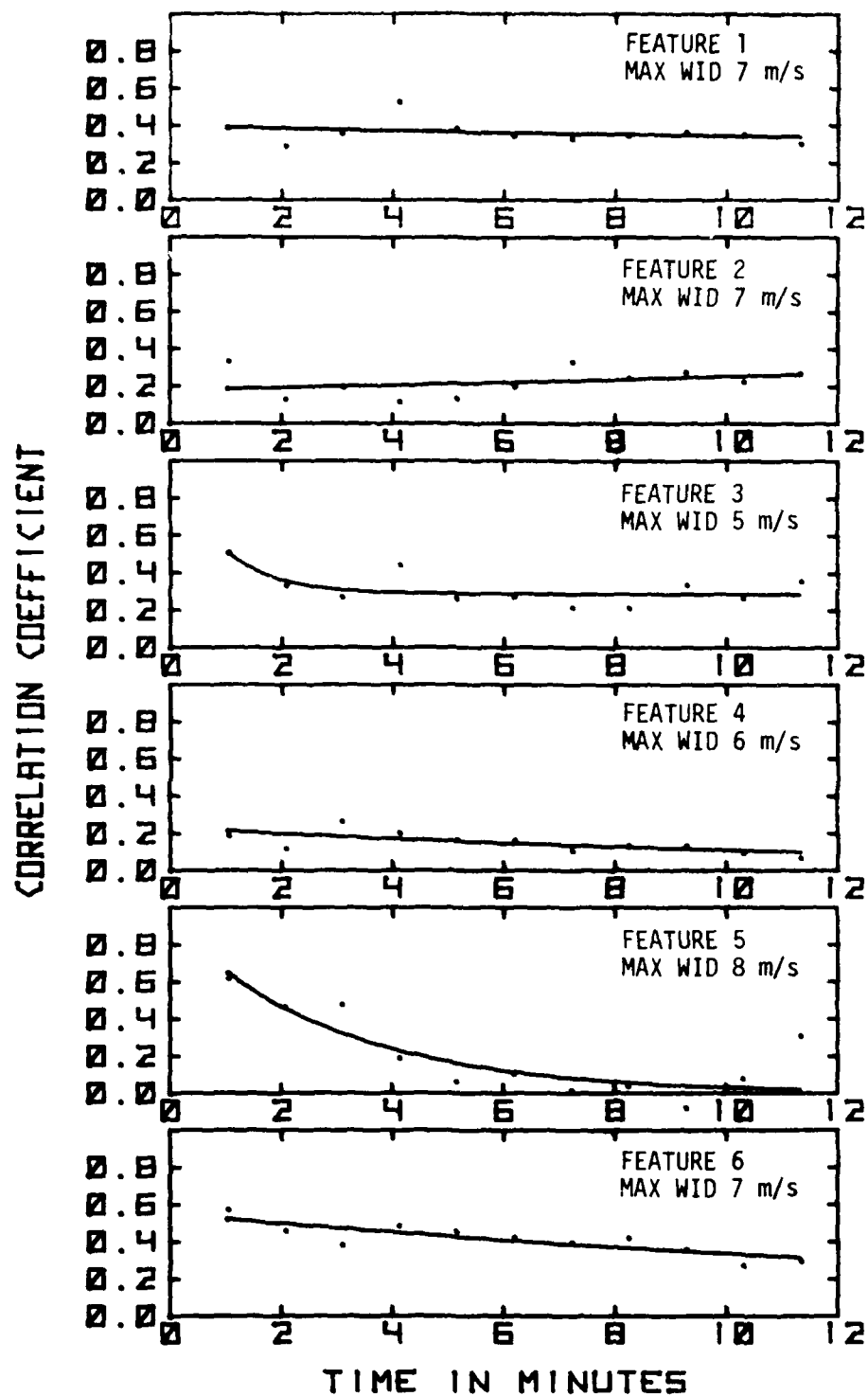
Figure 15(a)(iii) Spectrum width correlation evolution of April 24, 1980 storm at 0.4^\circ elevation.
