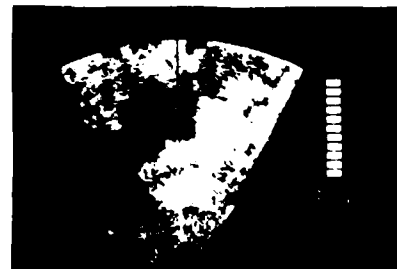
Figure 10(a) Spectral moment displays of June 17, 1980 storm at 0.4^\circ elevation. Reflectivity field was weak and nearly static. Hence only one representative frame is shown for reflectivity.
