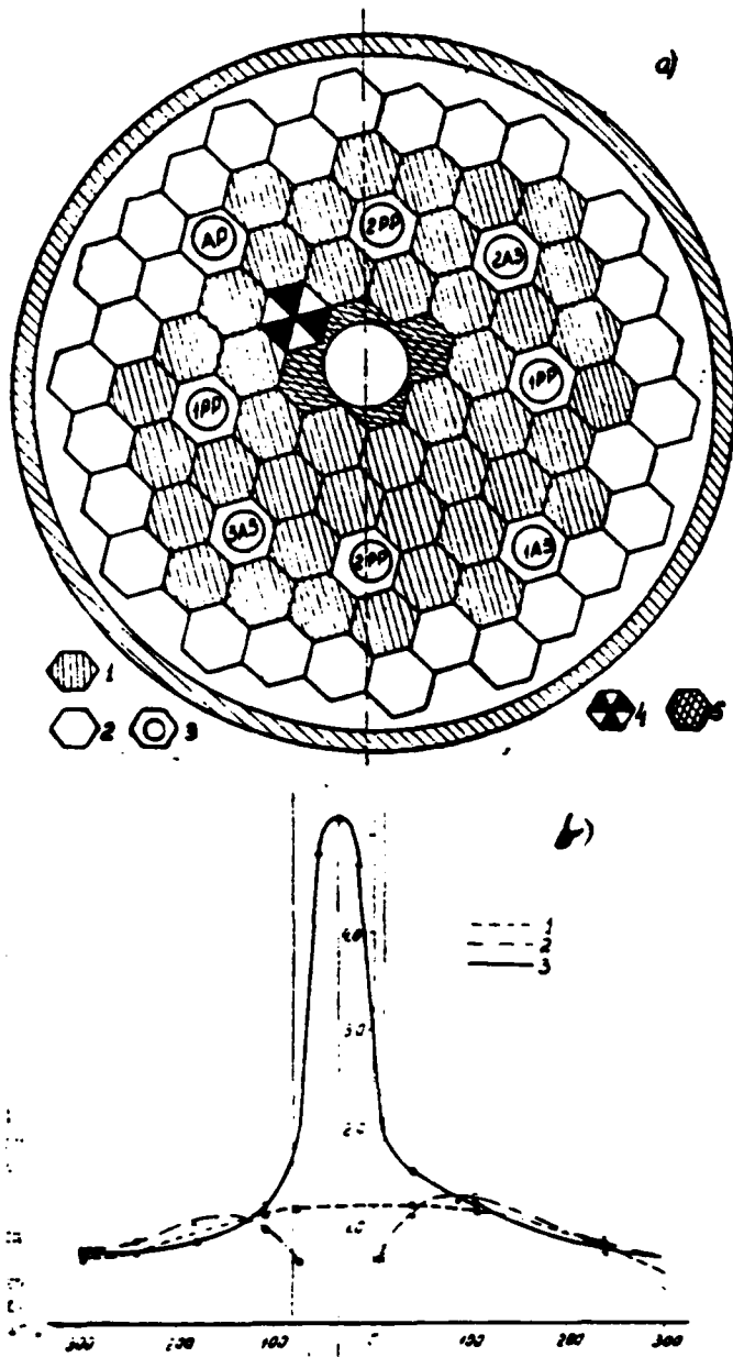
Fig. 1. a - cartogram representing loading of active zone for case of 90 mm central channel. 1 - type I fuel element; 2 - pump; 3 - safety and control organs; 4 - neutron source; 5 - pump with central channel; N_{kp} = 43 fuel elements; \Sigma_{PP+AP} = 8.5\% ; \Sigma_{AS} = 4.9\% ; b - distribution of thermal neutron flux over diameter of active zone (1 - air channel, 2 - physical mock-up of loop channel, 3 - "wet" channel).
