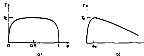
FIG. 9. (a) Coexistence curve for the monomer case ( M=1 ) and (b) for the polymer case ( M \gg 1 ).
