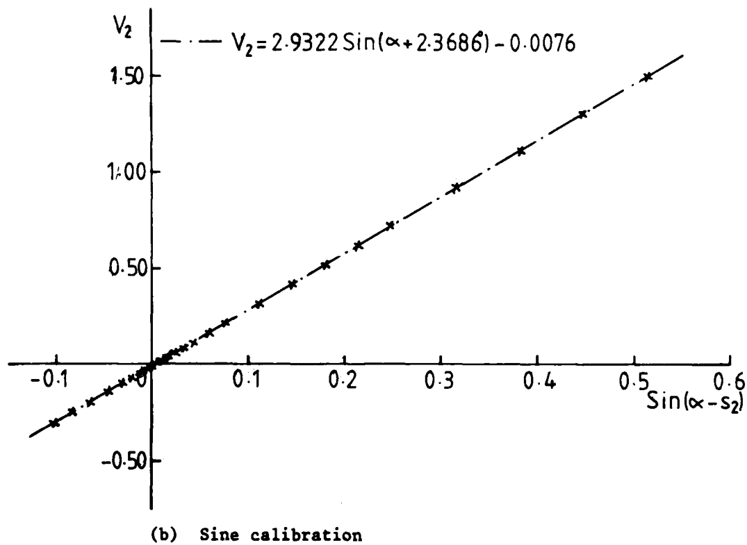
Fig 1a&b Accelerometer calibrations
