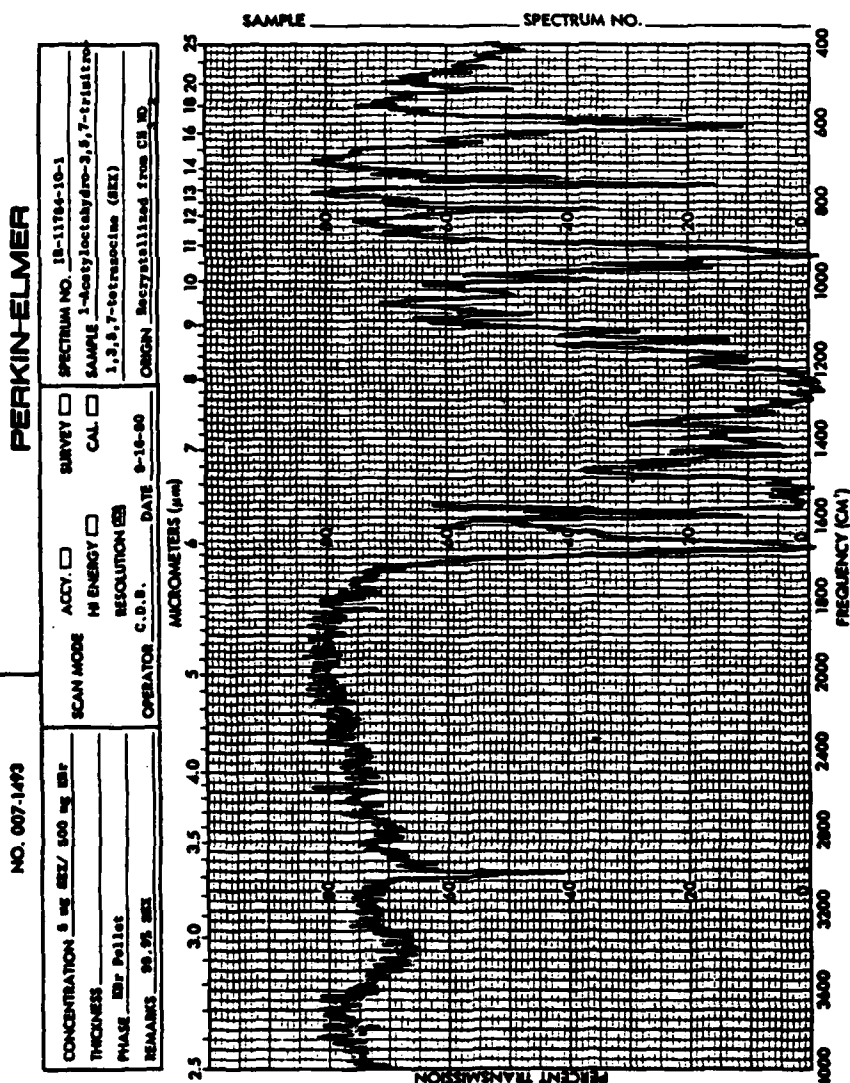
INFRARED SPECTRUM
