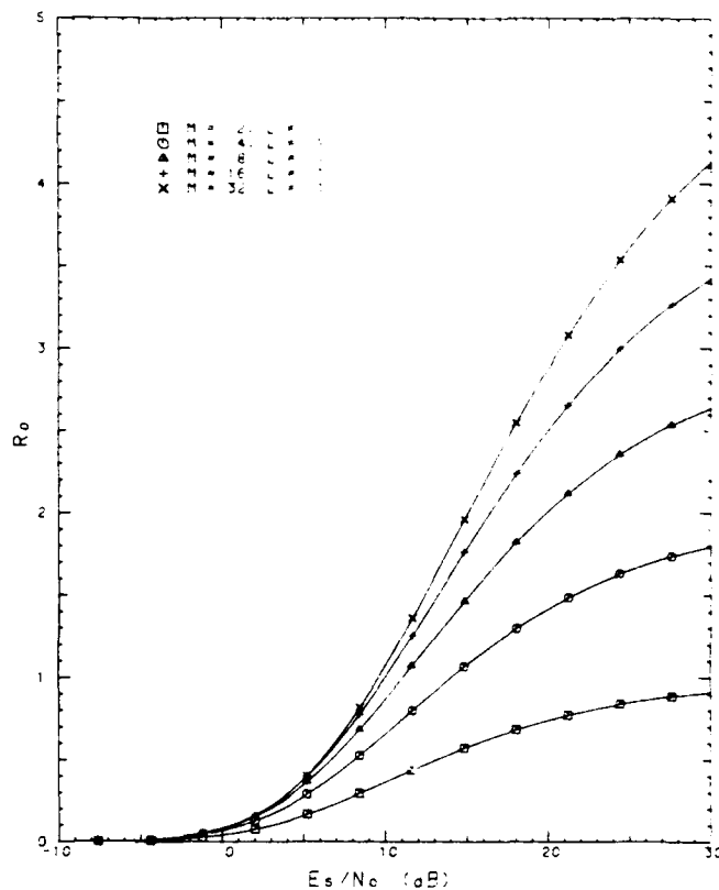
Fig. 24 — R_0 vs E_s/N_0 for Rayleigh fading channels
