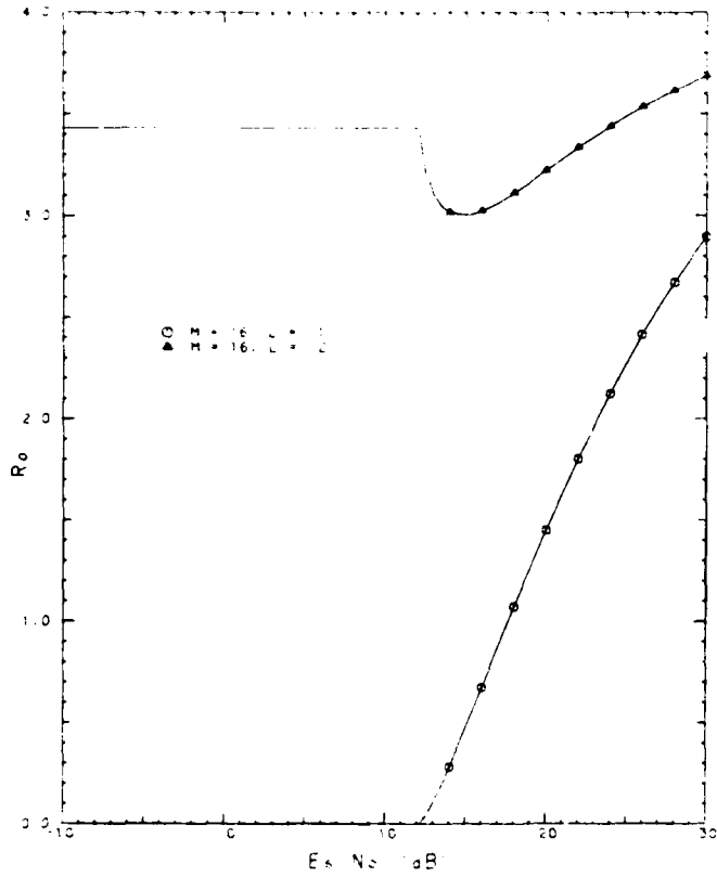
Fig. 10 — R_0 vs E_k/N_0 for optimal tone-jamming channel
