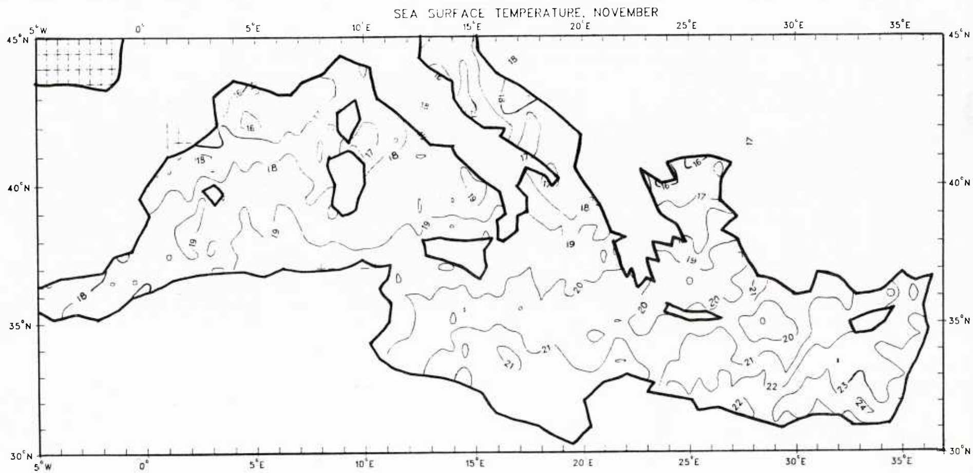
FIGURE 4-22: GDEM - NOVEMBER SEA SURFACE TEMPERATURE (SST) FOR THE MEDITERRANEAN SEA
