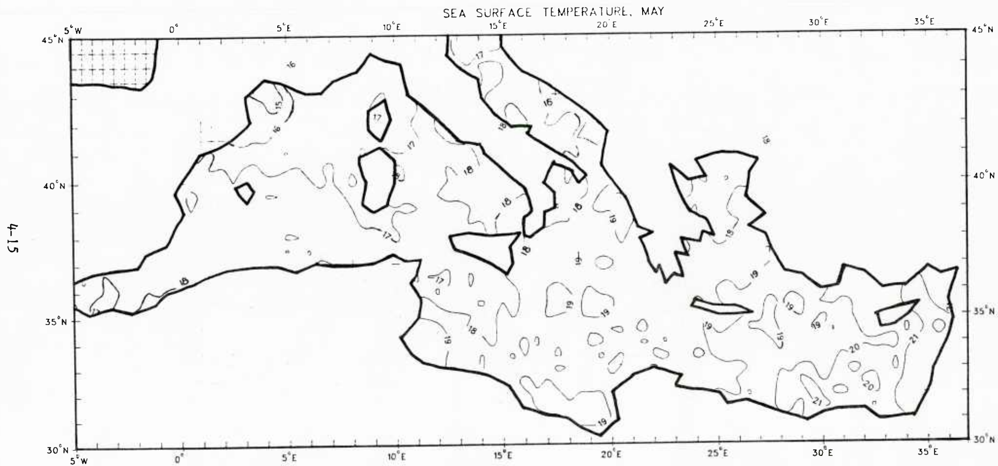
FIGURE 4-10: GDEM - MAY SEA SURFACE TEMPERATURE (SST) FOR THE MEDITERRANEAN SEA
