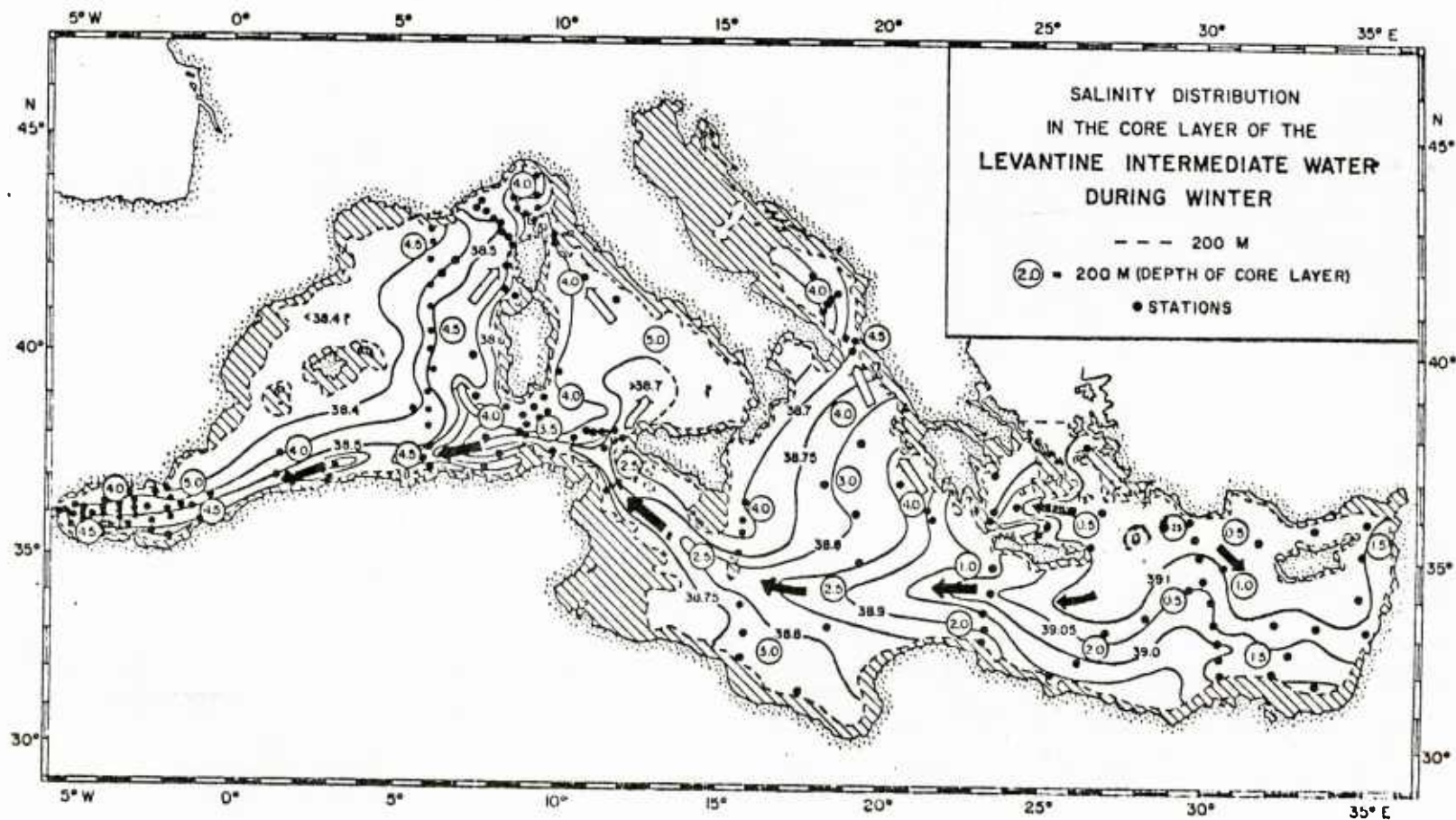
FIGURE 5-16: LOCATIONS OF THE SALINITY CORE LAYER WITHIN THE LEVANTINE INTERMEDIATE WATER IN THE WINTER (WUST, 1961)
