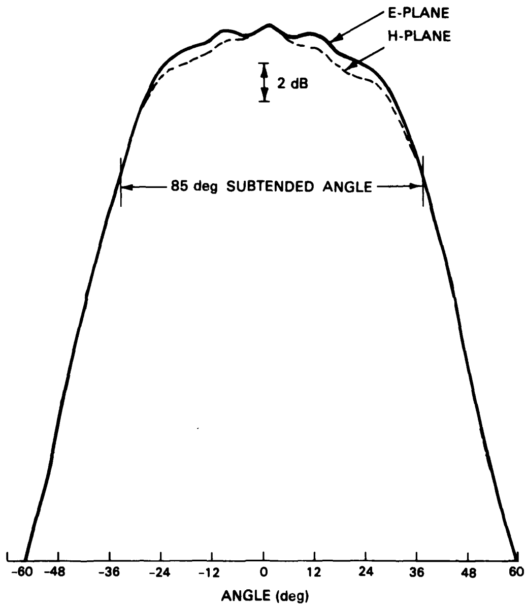
Fig. 6. Feed radiation patterns at 44.5 GHz.
