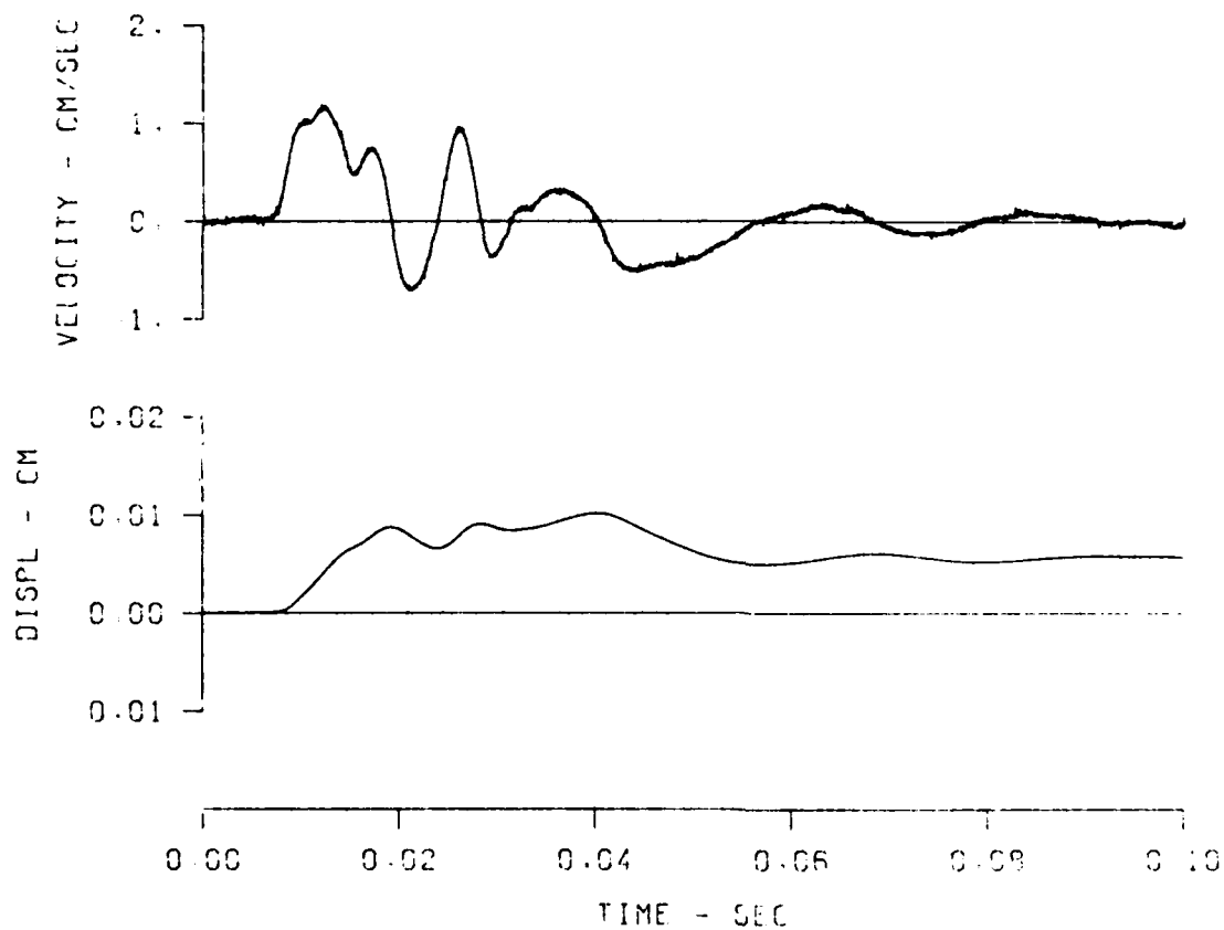
Figure B.8 Horizontal particle velocity measurement and integration, gage canister on rock at 73.2 ft slant distance.
