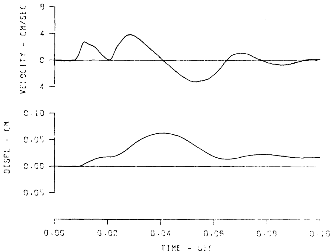
Figure B.1 Vertical particle velocity measurement and integration, gage canister on rock at 47.0 ft slant distance.
