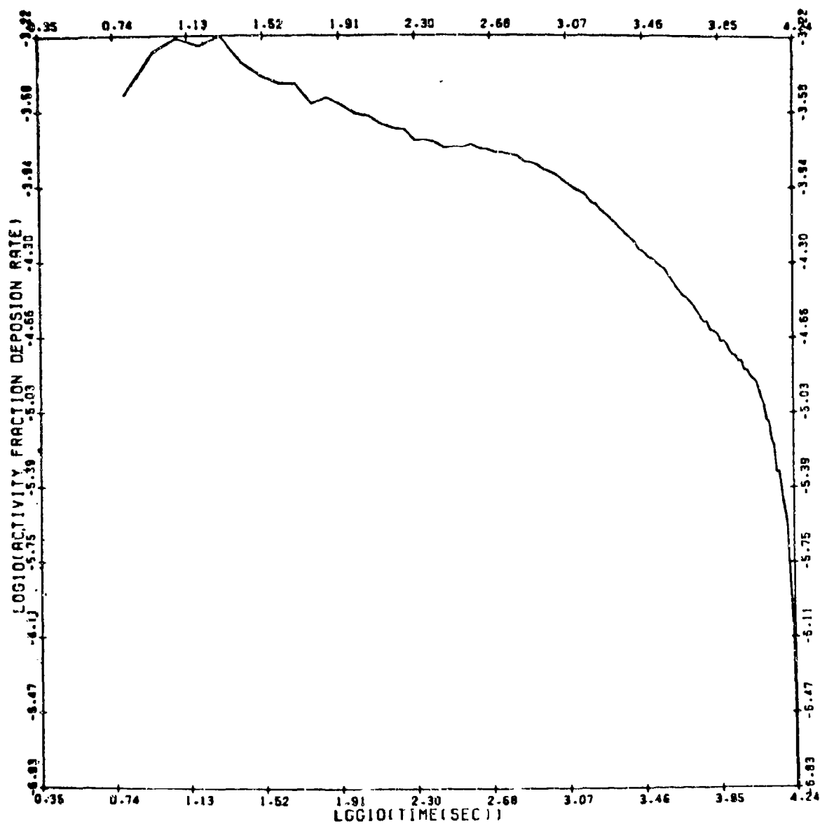
Figure 1. Computer plots of activity fraction deposition rate vs. time as computed by DEFFIC. (continued)
