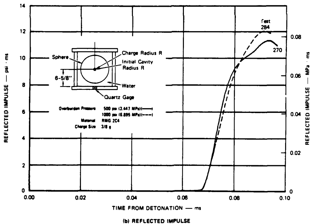
FIGURE C.1 REFLECTED PRESSURE AND IMPULSE FROM COUPLED CAVITY EXPLOSIONS—OVERBURDEN EFFECT
