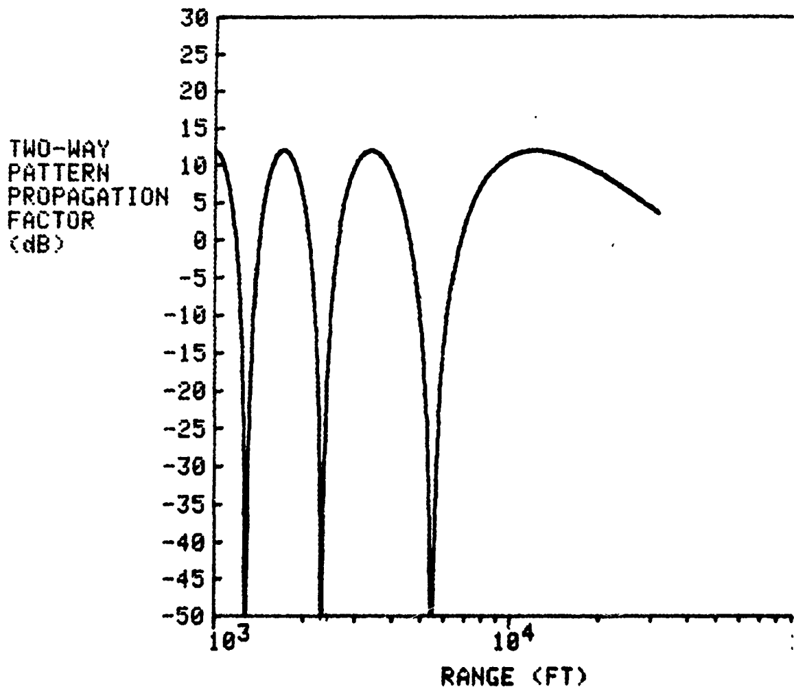
Figure 4.75. Theoretical Multipath Lobing Structure
