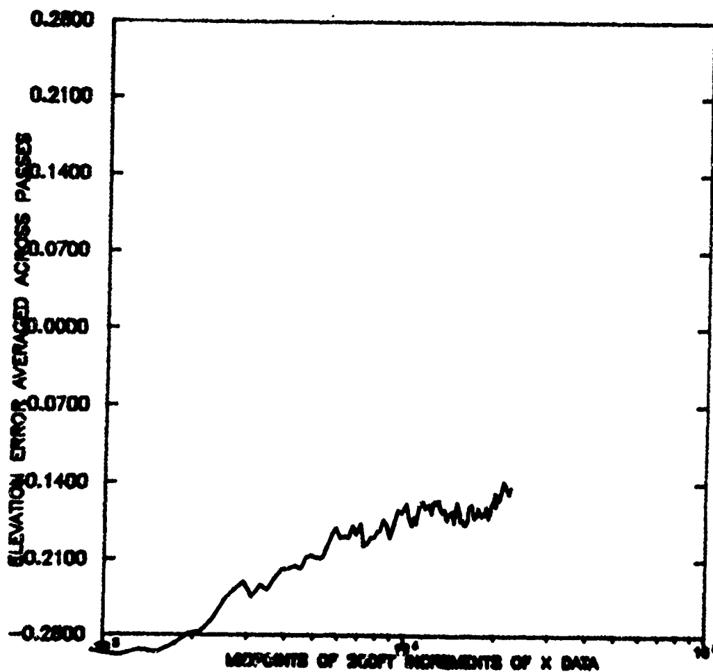
Figure 4.40. Elevation Error Averaged Across Passes, Configuration 2
