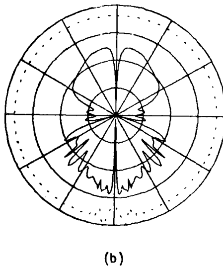
Figure 40. Azimuth plane pattern for \lambda/4 monopole mounted (a) forward of wings (b) over wings.
