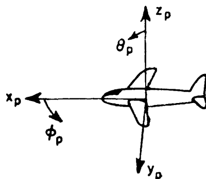
(b) ELEVATION PLANE COORDINATES ( \text{THC}=90^\circ , \text{PHC} = \pm 90^\circ )
