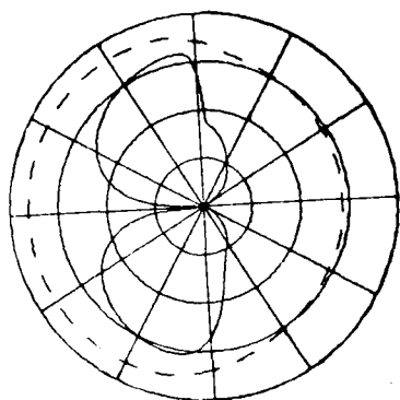
(a) \theta_c=0^\circ , \phi_c=90^\circ , \theta_p=90^\circ
