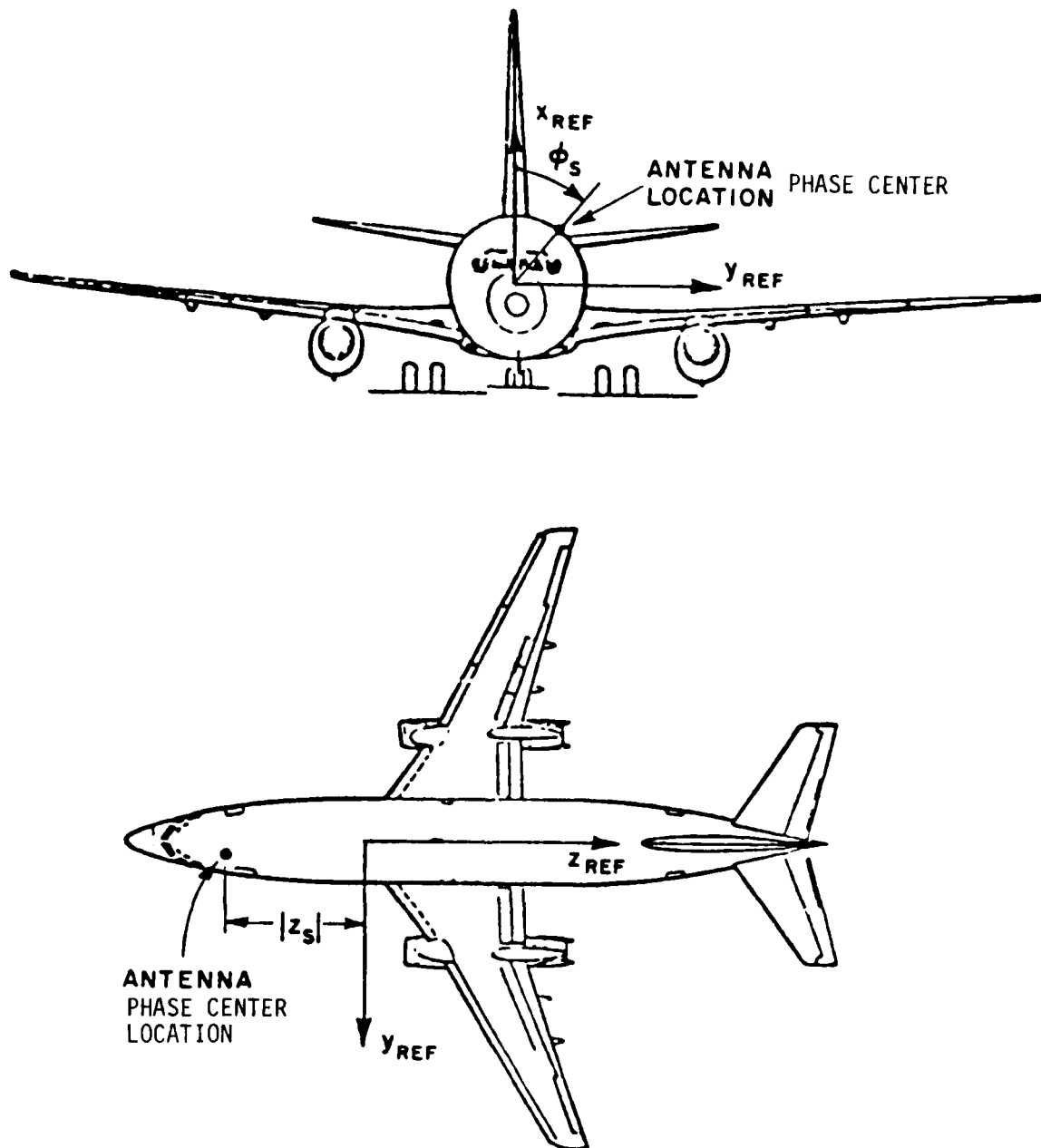
Figure 2. Definition of the antenna phase center location for computer code. Note that PHS = \phi_s and ZS = -|Z_s| in the above drawings.
