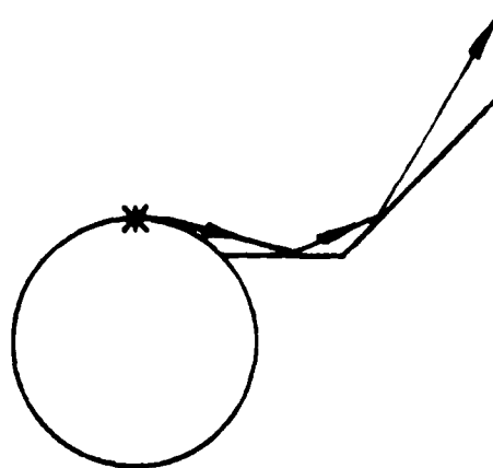
reflected-reflected field
