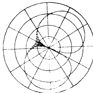
(b) \theta_c=90^\circ , \phi_c=0^\circ , \theta_p=90^\circ
