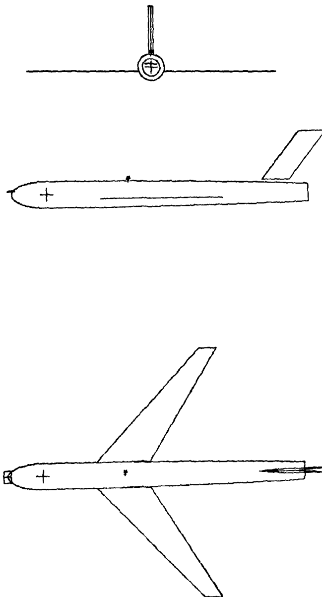
Figure 33. Computer simulated model of KC-135. (Antenna mounted over wings)
