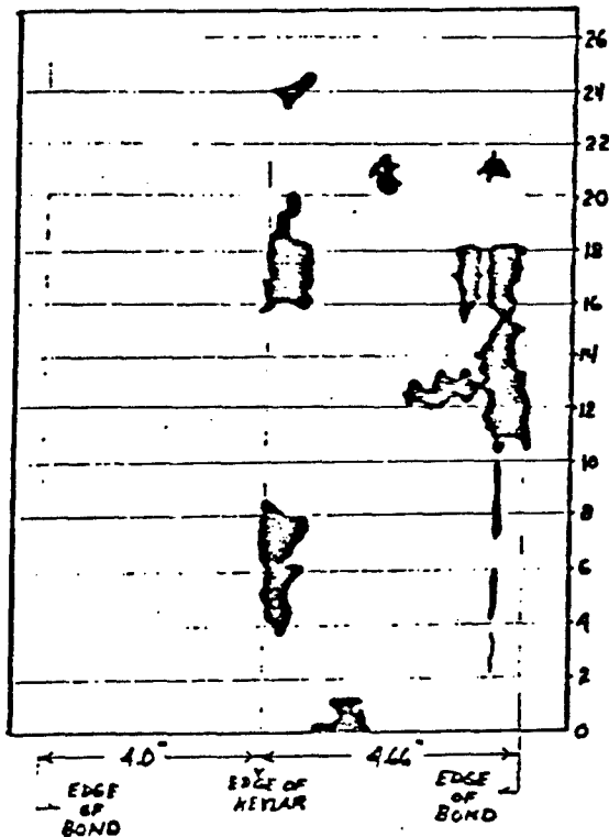
JOINT A
