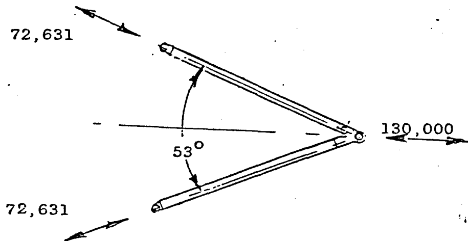
LOADING GEOMETRY
