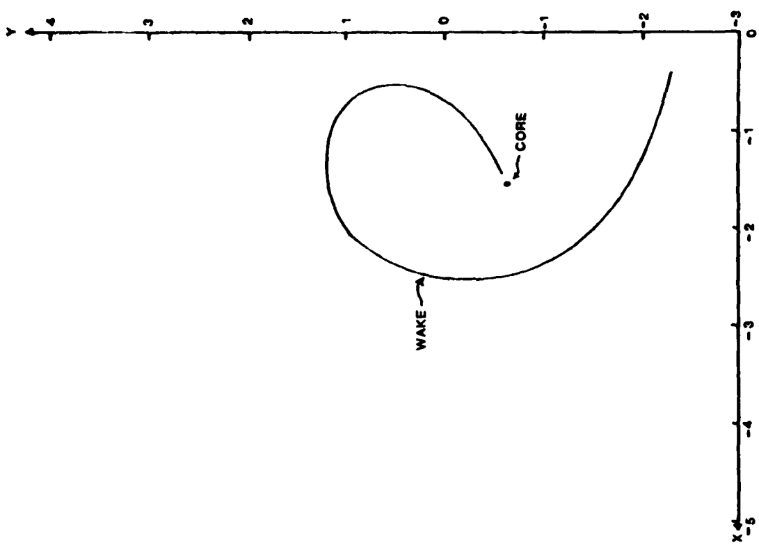
Figure 29. Bent Plate Wake Location, \alpha = 20^\circ and 6 Inches Downstream
