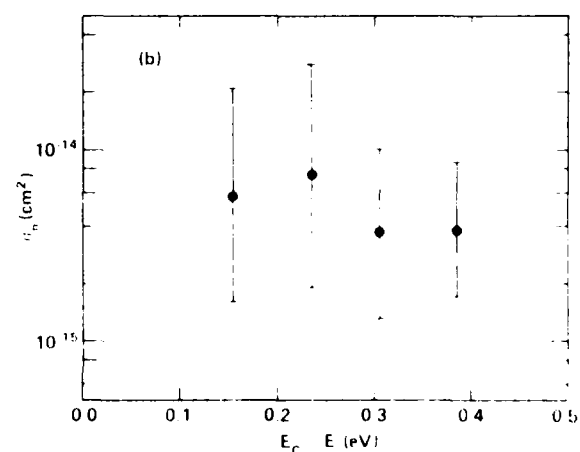
FIG. 9. Results for energy-resolved DLTS measurements of electron traps at the Si-SiO 2 interface: (a) mean Fermi energy \langle F_p \rangle for maximum net emission signal \Delta V_{GG, \max} vs temperature and (b) electron capture cross section \sigma_n vs energy in the silicon bandgap.
