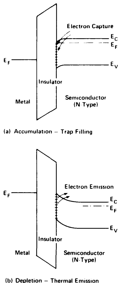
FIG. 1. Energy-band diagrams for an MIS device on an n -type semiconductor for (a) pulsed accumulation bias and (b) nonequilibrium depletion bias.
