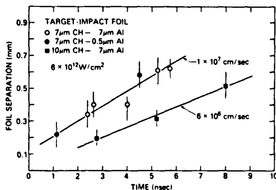
FIG. 6. A graph of target-impact foil separation versus the time (with respect to an arbitrary origin) at which the impact foil reacts to its collision with the target. The slopes of lines drawn through points accumulated over many discharges give the dense target velocities. The laser pulse duration is 4-nsec FWHM.
