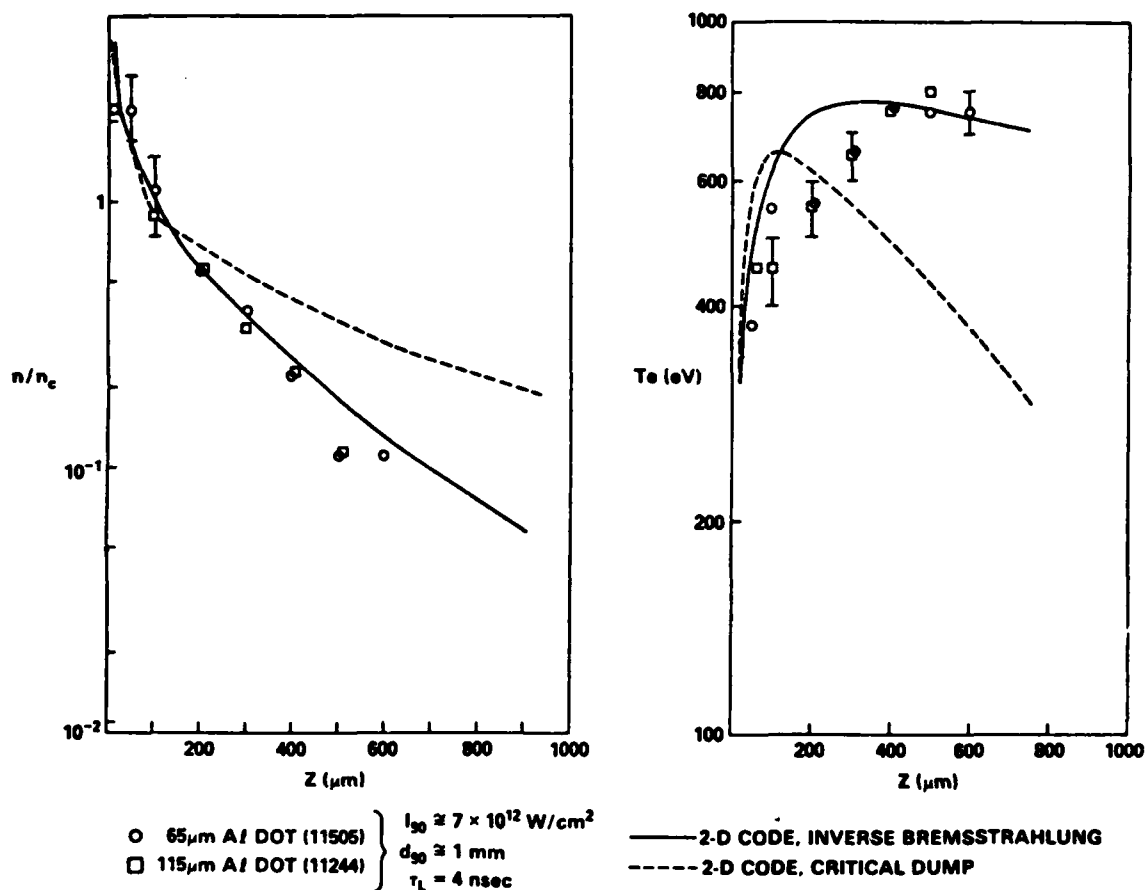
Fig. 9 Data points show density and temperature profiles from spot spectroscopy with 65 \mu\text{m} (o) and 115 \mu\text{m} (□) diameter Al dots. Experimental conditions are I_{90} \approx 7 \times 10^{12} \text{ W/cm}^2 within d_{90} \approx 1 \text{ mm} . 2-D code calculations for the same conditions are shown by the solid curve. The sensitivity of the agreement between code and experiment to details of the code physics is shown by the dotted curve, generated with the 2-D code altered to neglect inverse bremsstrahlung and to dump all energy at critical density.
