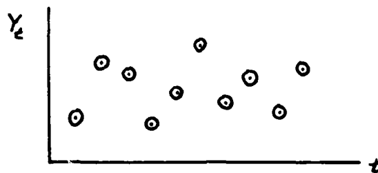
Figure 1: A No Trend Situation
