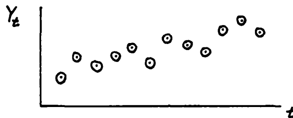
Figure 2: A Linear Trend Situation
