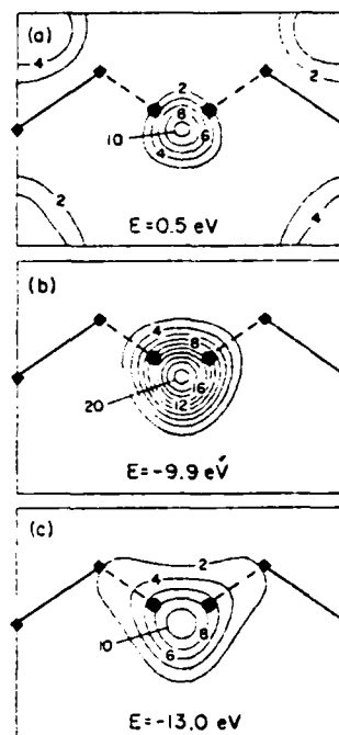
FIG. 7. Contour plots in the (110) plane of the three hydrogen-derived states at the zone center of the H-saturated Si vacancy superlattice. The charge density is normalized to one electron per superlattice unit cell.
