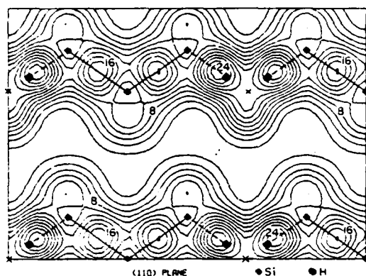
FIG. 1. Contour plot in the (110) plane of the pseudo-charge-density of the H-saturated Si vacancy. The units are electrons per diamond-lattice unit cell. Solid straight lines denote Si-Si bonding directions and dashed lines indicate H-Si bonds; crosses denote vacant Si sites. For clarity the abscissa and ordinate lengths are 1.5 times the corresponding supercell dimension.
