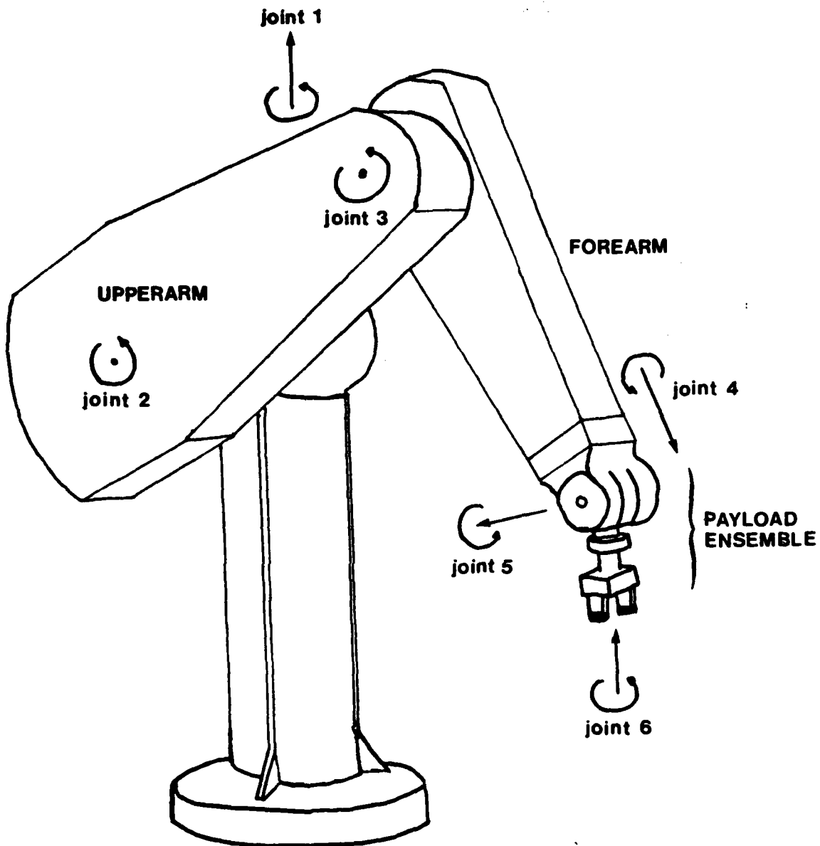
Figure 2. The PUMA has six revolute joints. It can be decomposed into three components: the upperarm, the forearm, and the combined wrist, hand and payload.
