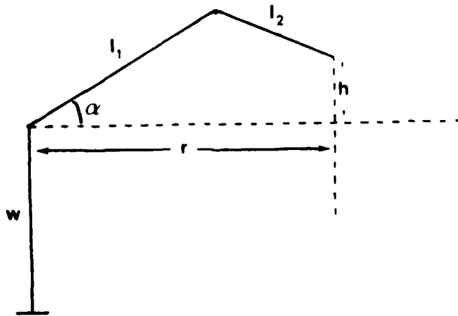
Figure 27. A side view of the manipulator kinematics.
