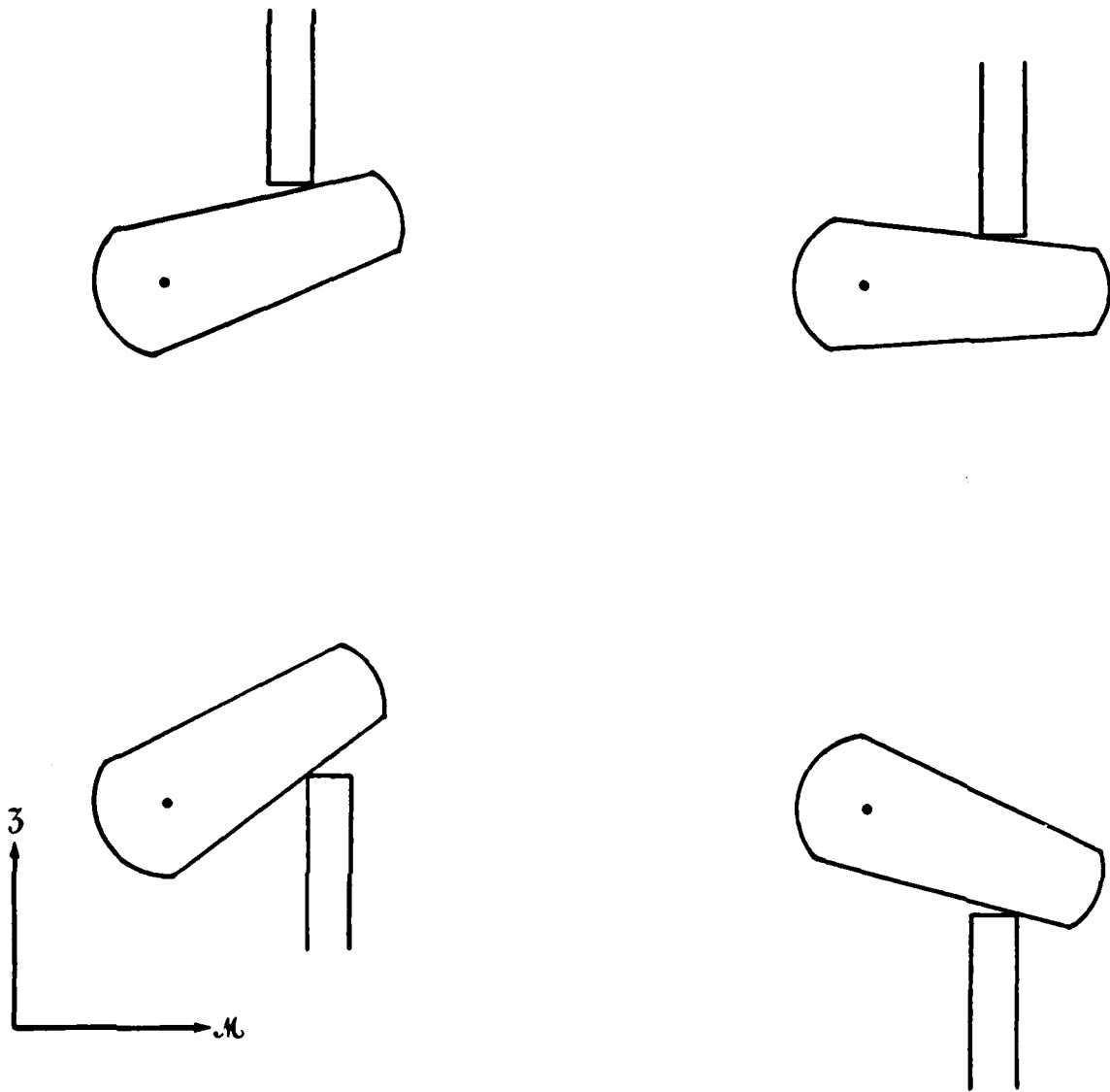
Figure 23. The four ways the upperarm can hit an obstacle with one of its upper or lower surfaces.
