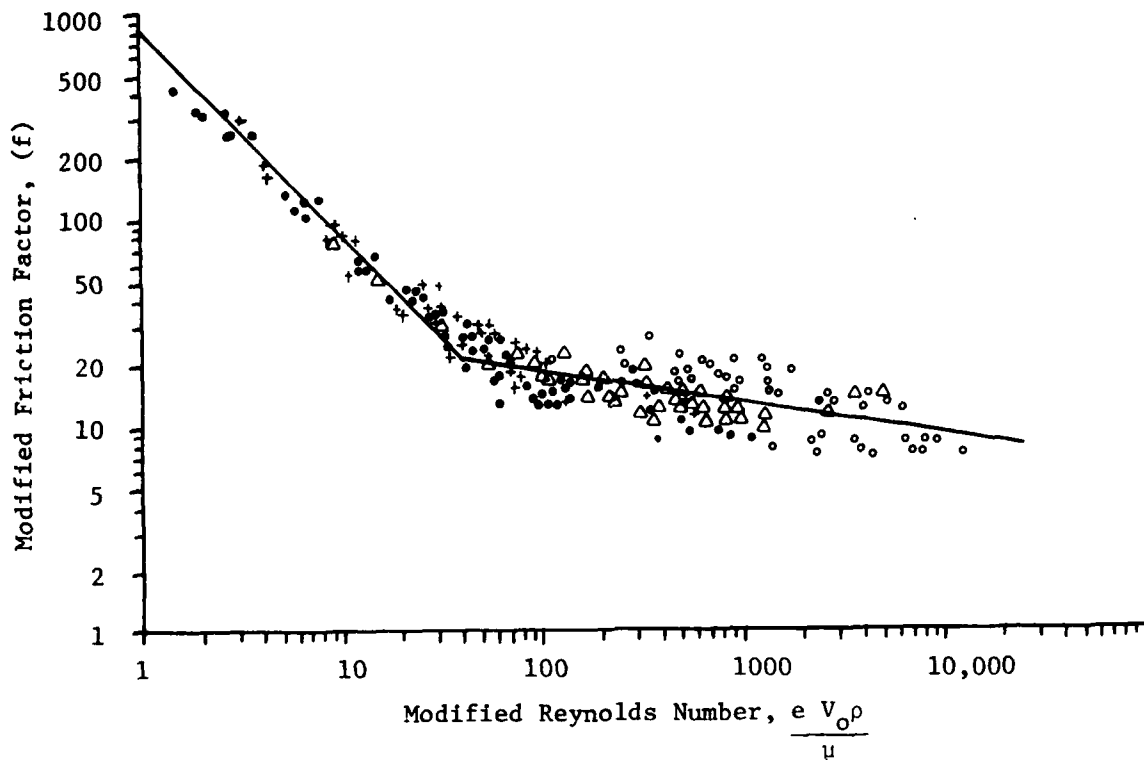
FIGURE 17. CORRELATION OF DATA ON PRESSURE DROP THROUGH BEDS OF SOLIDS
