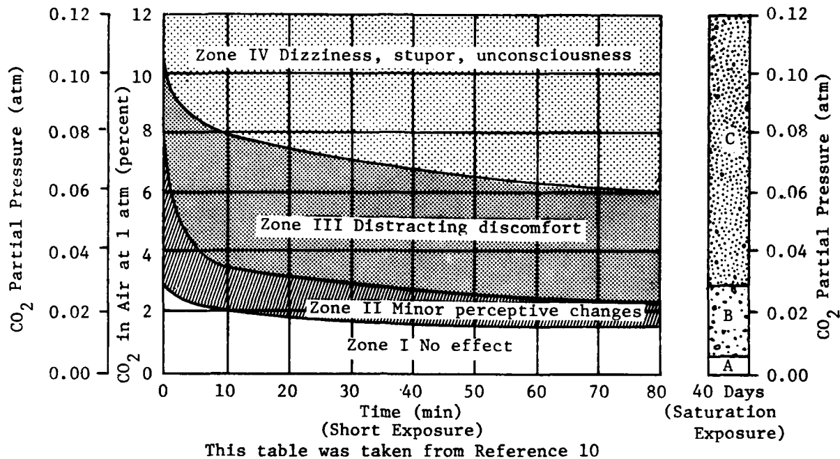
FIGURE 1. RELATION OF PHYSIOLOGICAL EFFECTS TO CARBON DIOXIDE CONCENTRATION AND EXPOSURE PERIOD
