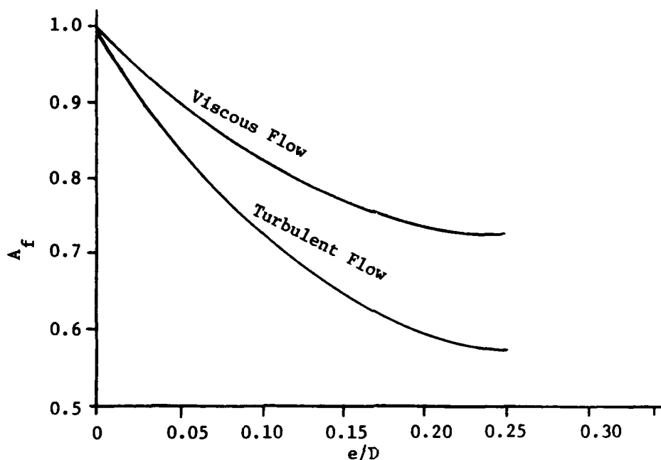
FIGURE 18. WALL EFFECT FACTOR
