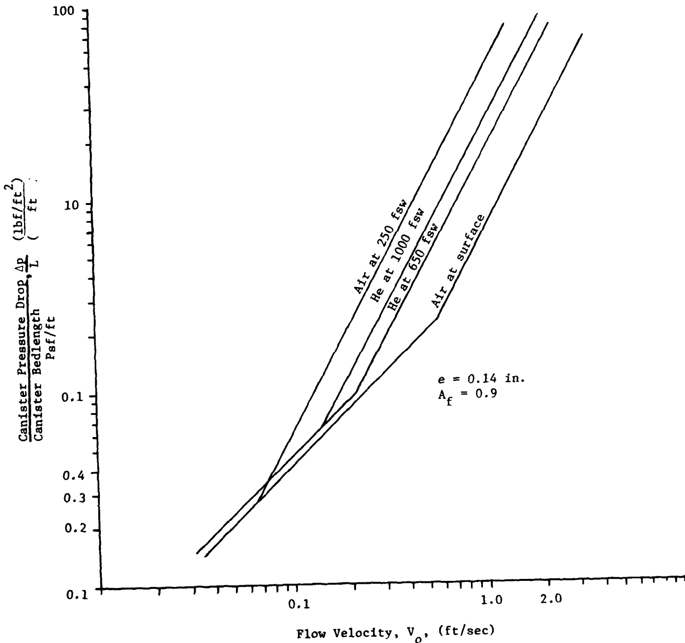
FIGURE 19. PRESSURE DROP ACROSS ABSORBENT CANISTERS AT VARIOUS DEPTHS
