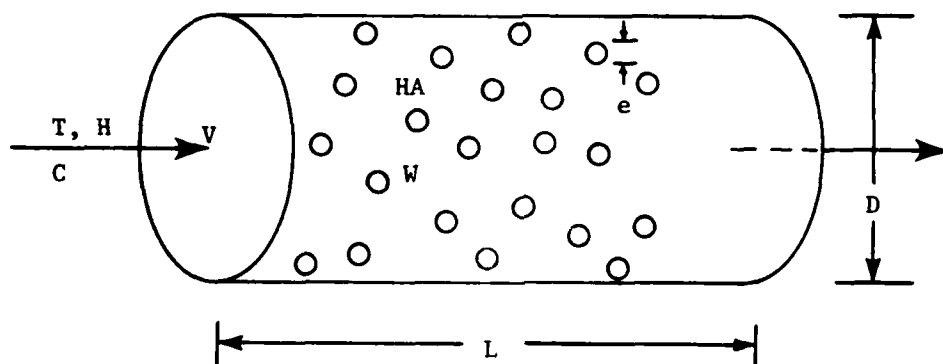
FIGURE 3. THE ABSORPTION PROCESS
