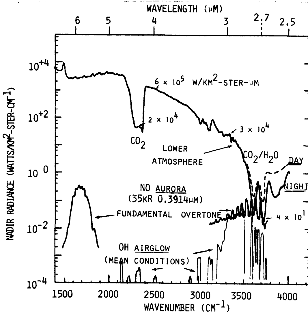
Figure 3. Infrared spectral radiances in the nadir of the mean hydroxyl vibrational-bands airglow, the nitric oxide emissions in 35 kR 0.3914 \mu m aurora, and the thermal emission and sunlight backscatter-int of the lower atmosphere (midlatitude summer conditions, 60° solar zenith angle in the daytime (dashed) curve). Spectral resolution of the thermal background is 20 \text{cm}^{-1} (LOWTRAN), of the airglow-aurora \sim 10 \text{ cm}^{-1} . Note: These are nominal, model values intended to provide a semiquantitative comparison of atmospheric background intensities; refer to the text.
