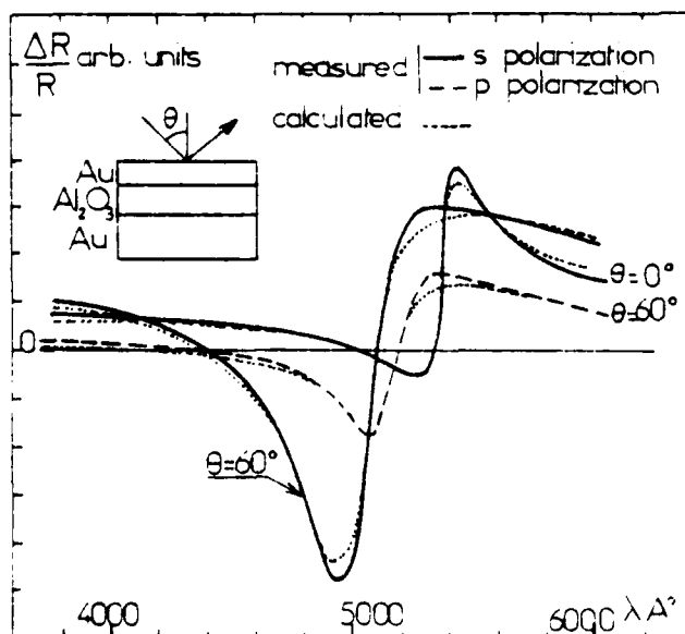
Measured and calculated E.R spectra of Au-Al 2 O 3 -Au structures
