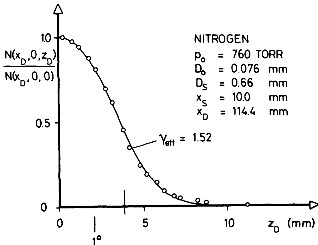
Figure 8: Match of predicted to observed nitrogen data
