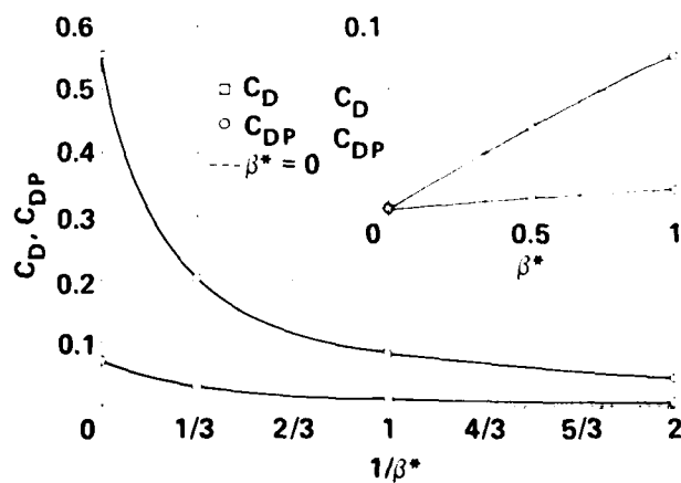
Figure 7: Drag coefficient versus 1/\beta^* for the case explained in Figure 6.
