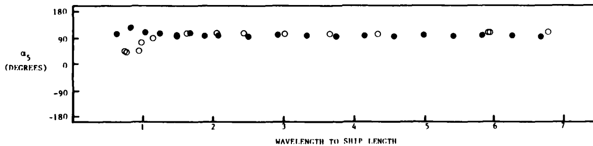
Figure 3h - Pitch Moment for F_n = 0.0 in Following Waves
