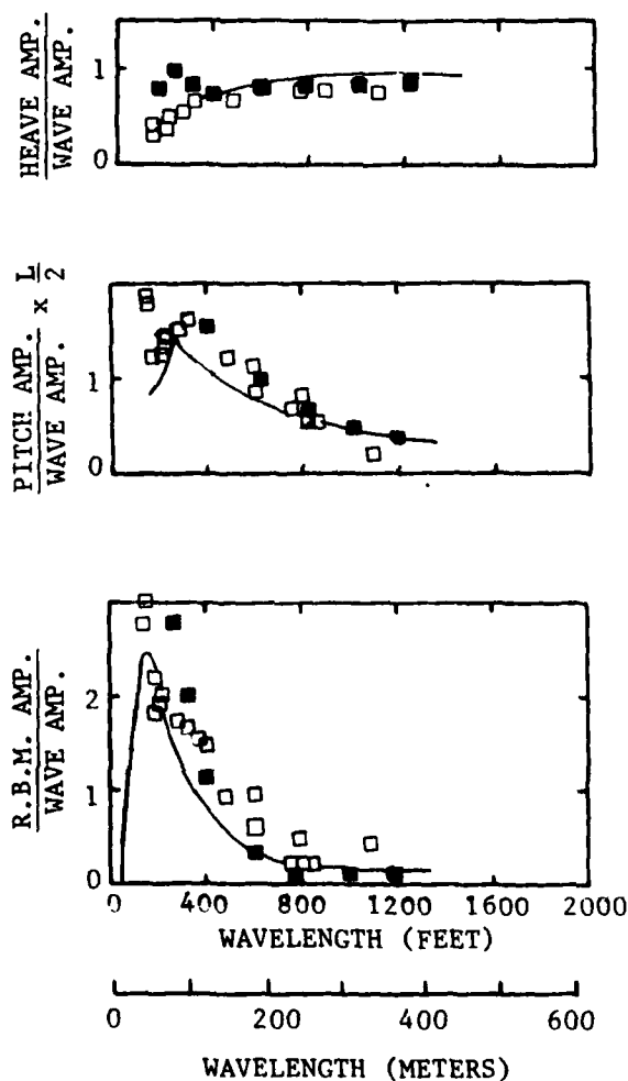
Figure 5d - Responses at 20 Knots in Bow and Quartering Waves
