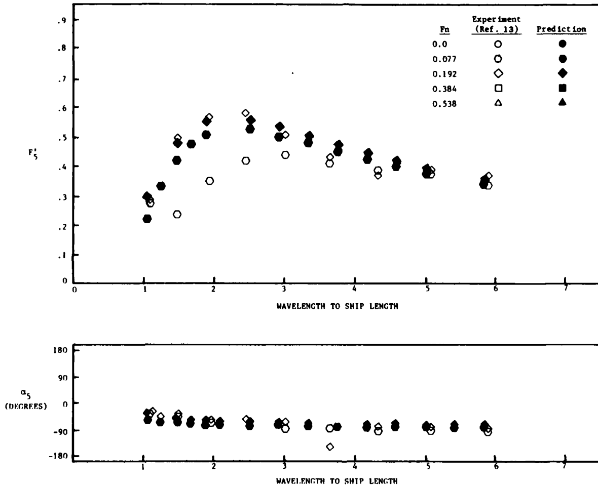
Figure 3d - Pitch Moment at F n = 0.077 and 0.192 in Head Waves
