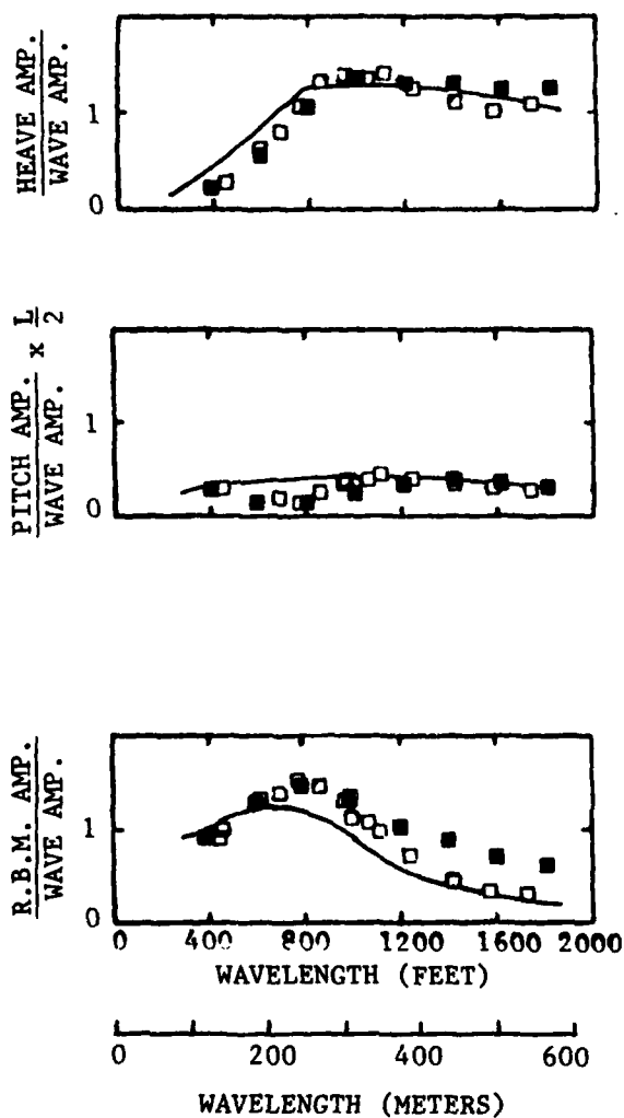
Figure 5d - Responses at 20 Knots in Bow and Quartering Waves
