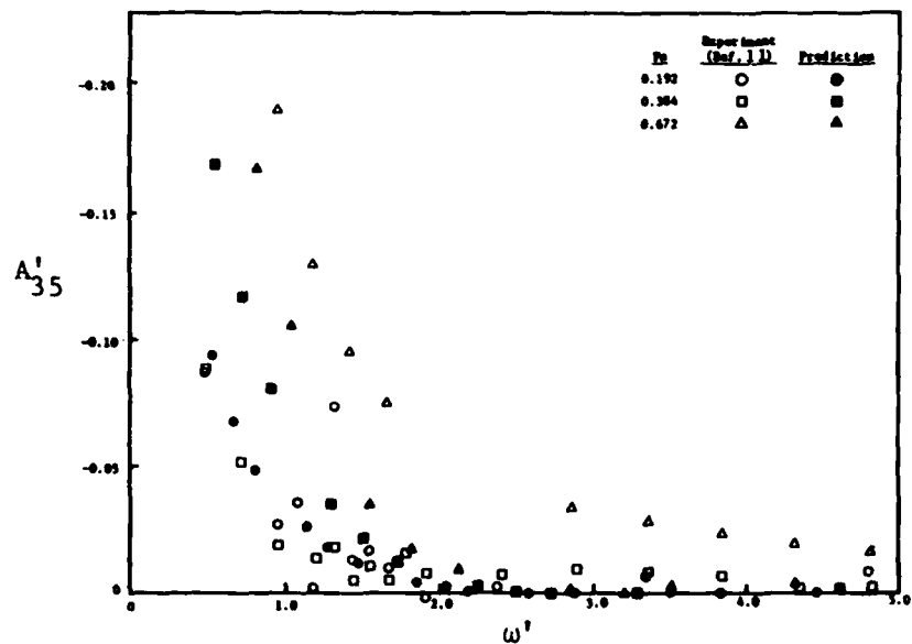
Figure 1b - Added Mass Coefficients A'_{55} and A'_{35}
