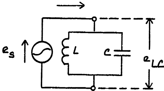
(b) Parallel - Tuned Circuit
