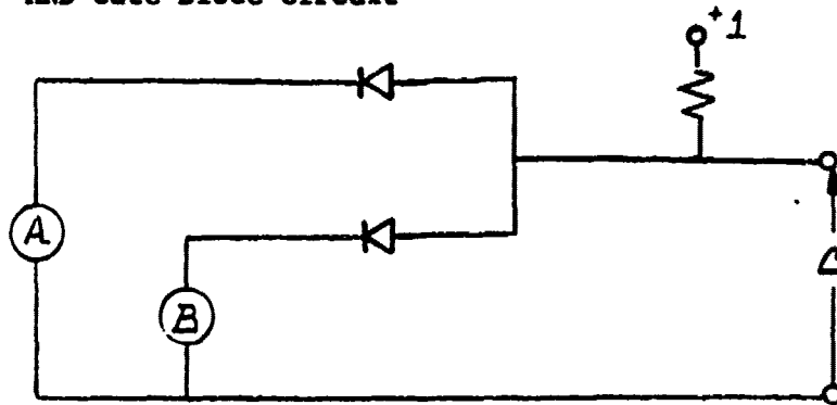
Figure 2.2.12.5 — AND Gate
