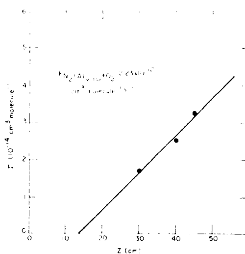
FIG. 8. Decay constants for N_2(A_{1g}) removed by O_2 as a function of mixing distance, P = 1.33 \text{ Torr} , \bar{v} = 1350 \text{ cm}^{-1} .
