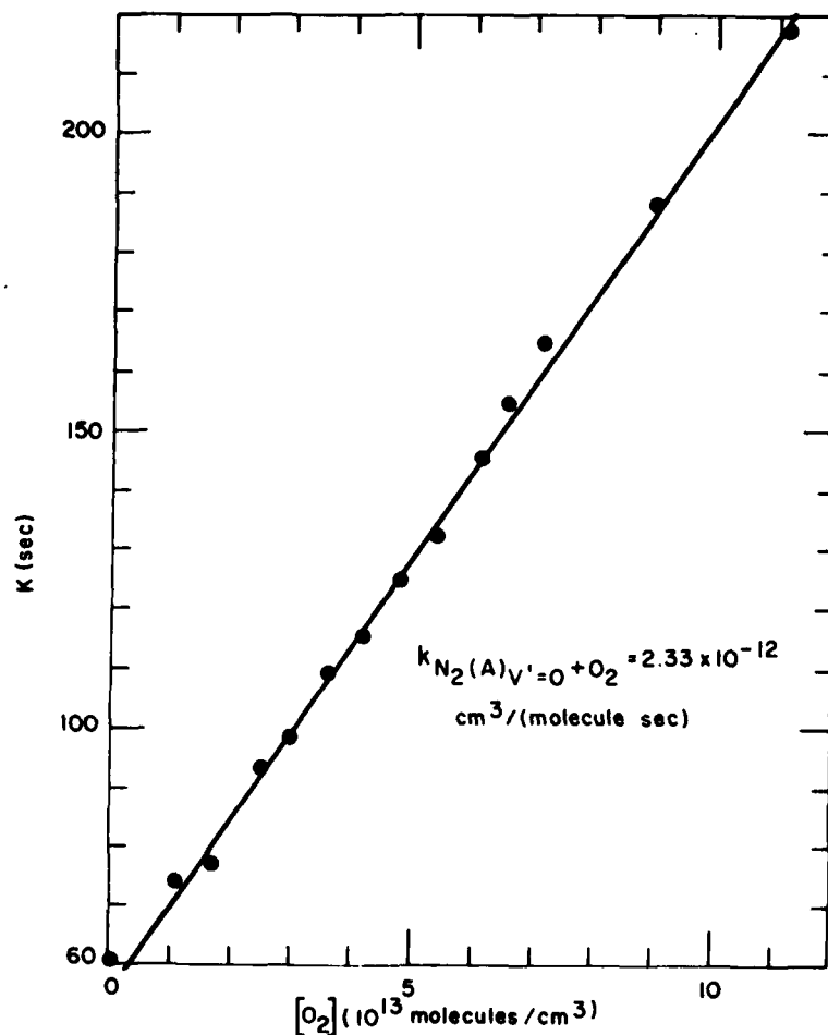
Figure 5. N_2(A)_{v=0} Decay Rates as a Function of [O_2] . P = 1.33 Torr
