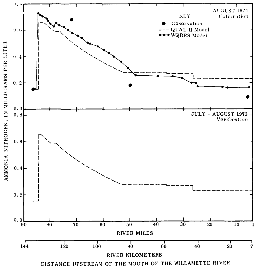
Figure 31. Observed and predicted ammonia-nitrogen, Willamette River
