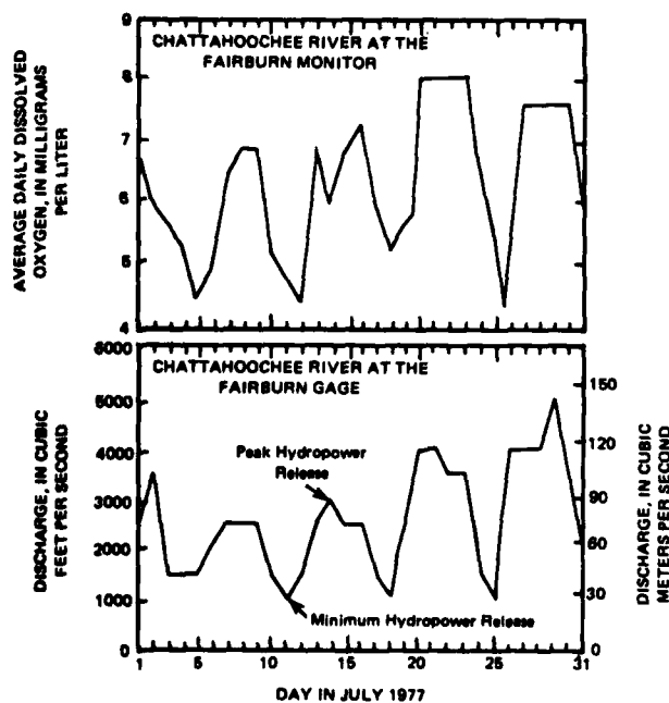
Figure 10. Dissolved-oxygen concentrations and mean daily discharge during 1977
