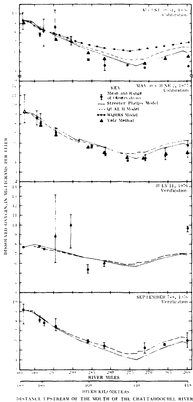
Figure 24. Observed and predicted dissolved oxygen, Chattahoochee River
