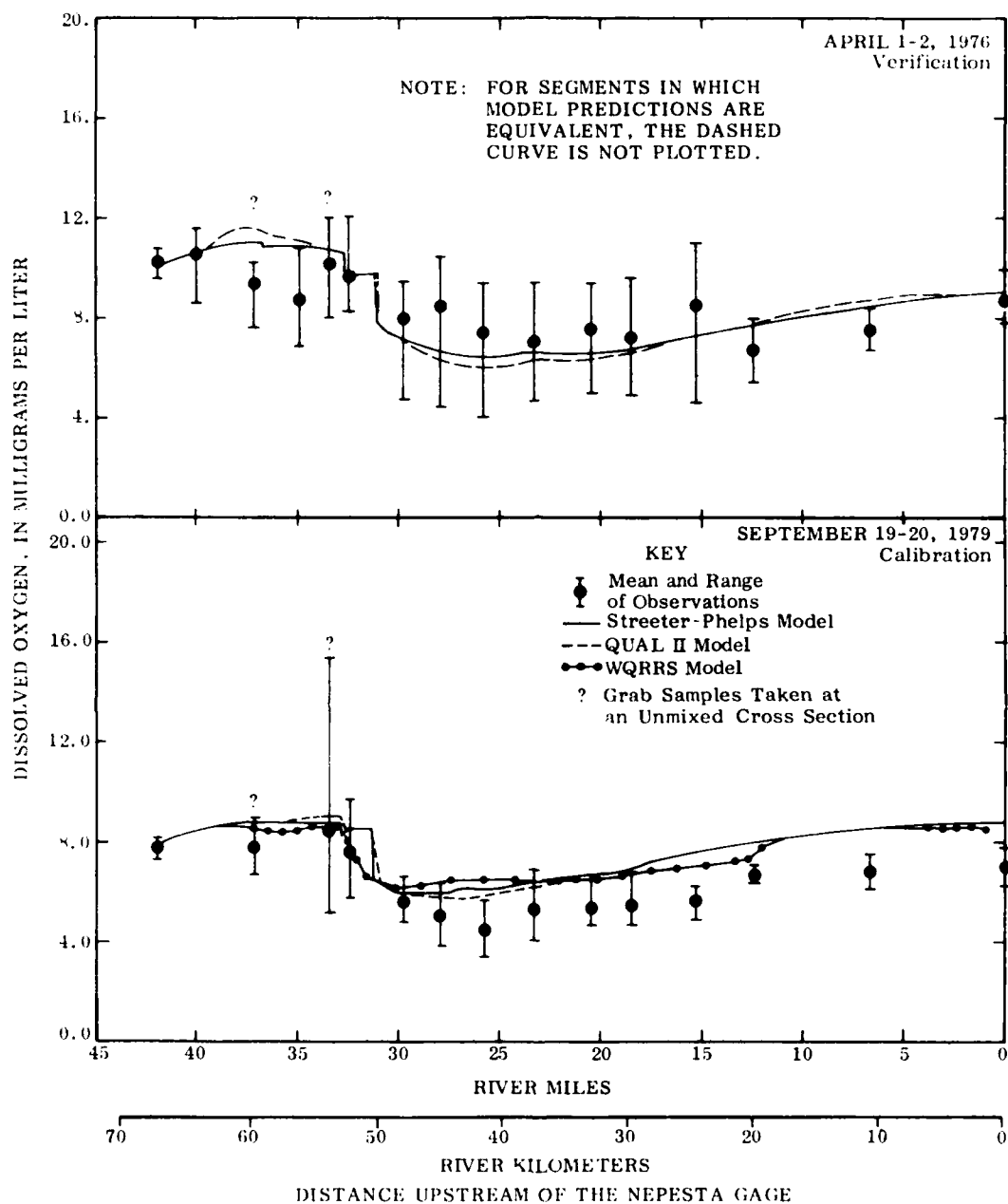
Figure 40. Observed and predicted dissolved oxygen, Arkansas River
