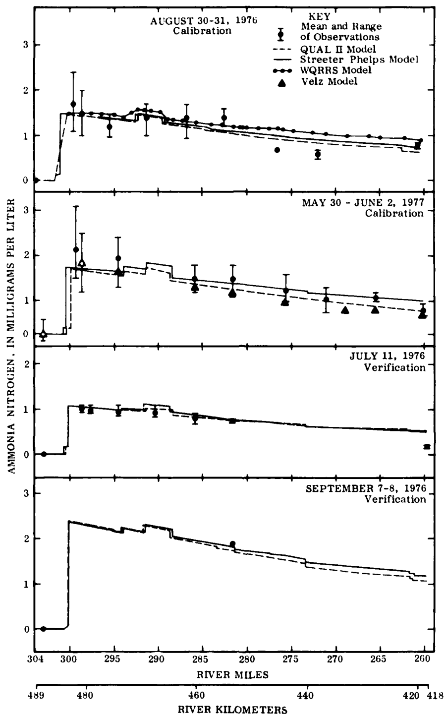
Figure 22. Observed and predicted ammonia-nitrogen, Chattahoochee River
