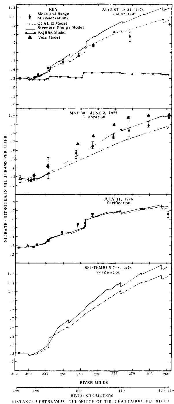
Figure 23. Observed and predicted nitrate-nitrogen, Chattahoochee River
