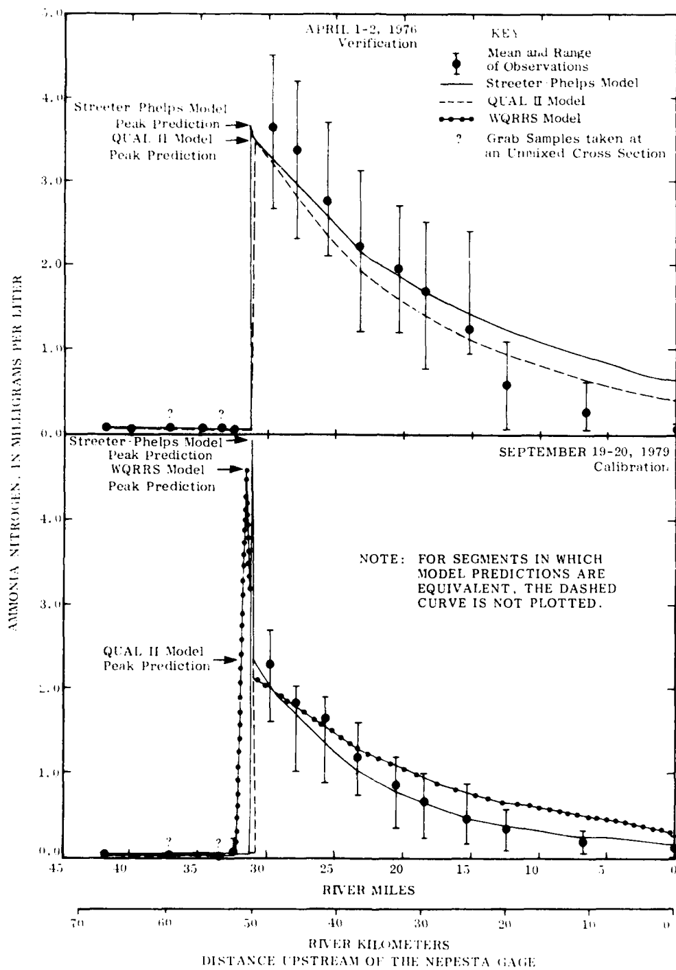
Figure 37. Observed and predicted ammonia-nitrogen, Arkansas River
