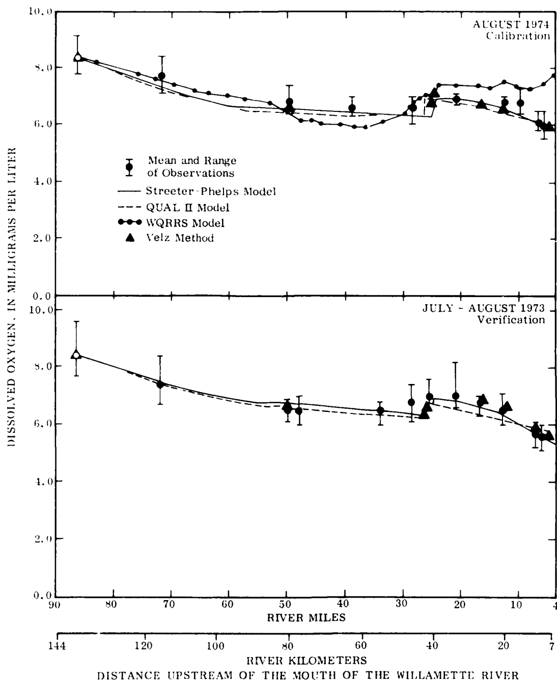
Figure 33. Observed and predicted dissolved oxygen, Willamette River
