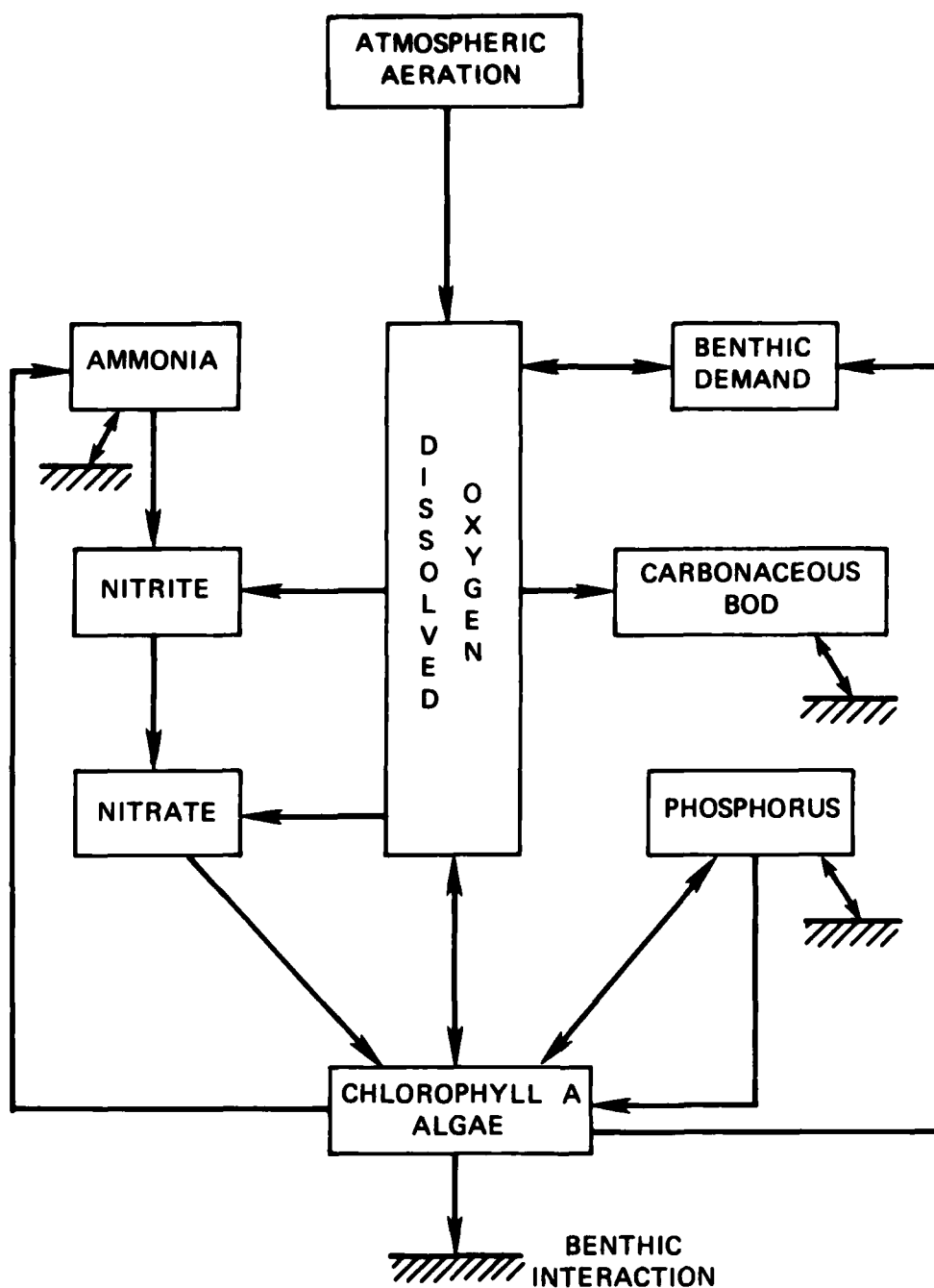
Figure 4. Water quality constituents modeled by the QUAL II model (adapted from Roesner, Giguere, and Evenson, 1977A)
