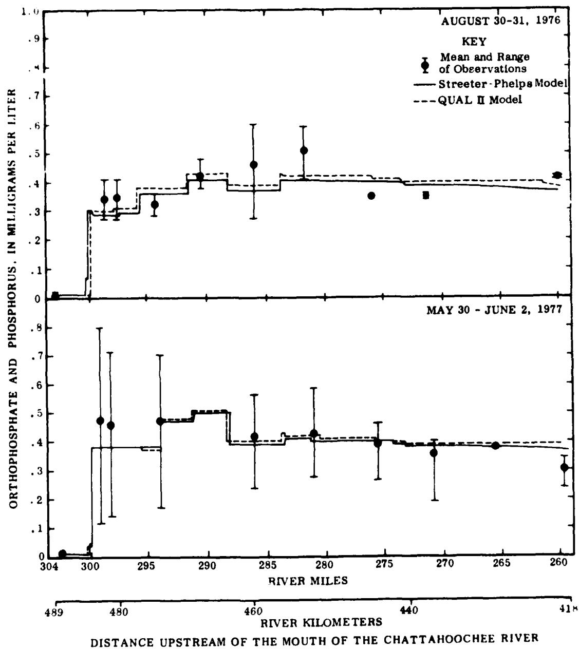
Figure 25. Observed and predicted orthophosphate and phosphorus, Chattahoochee River
