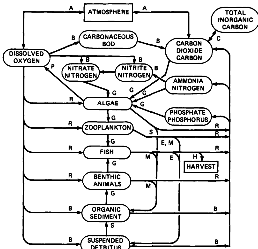
Figure 6. Ecologic and water quality relationships modeled by the WQRRS model (adapted from Smith, 1978)
