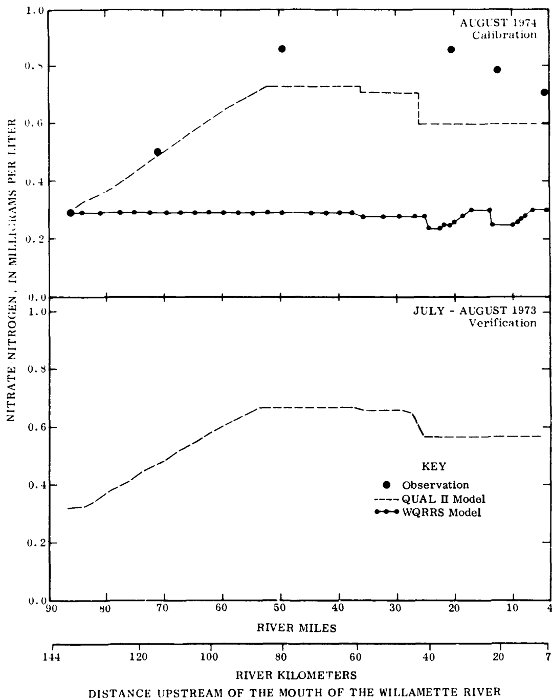
Figure 32. Observed and predicted nitrate-nitrogen, Willamette River
