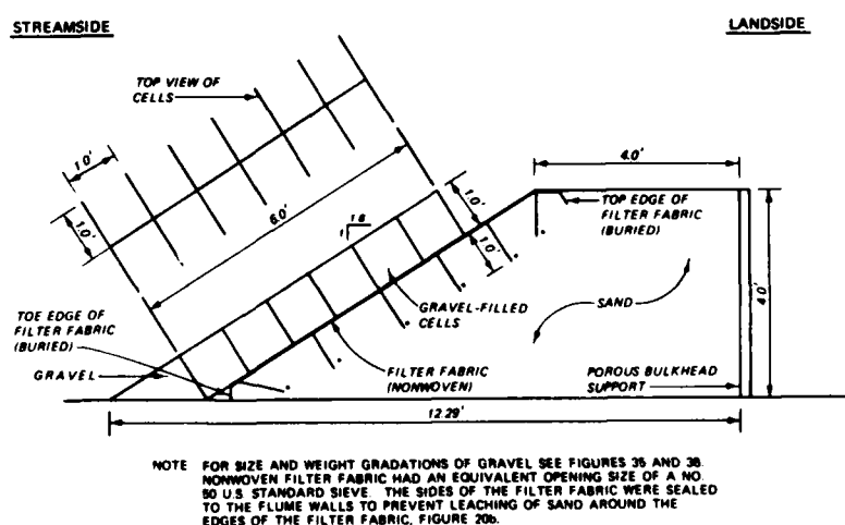
Figure 39. Plan 8C, sand streambank with gravel-filled cells and nonwoven filter fabric protection
