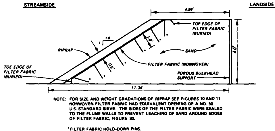
Figure 25. Plan 6, sand streambank with 0.5 ft of riprap and nonwoven filter fabric protection
