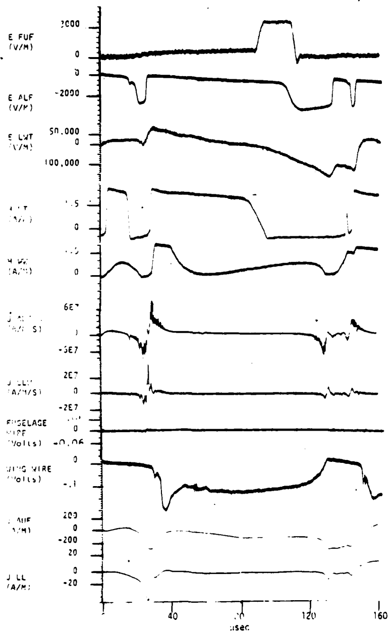
Figure 78. A 164 \mu sec Data Window that Includes the Largest Pulse in the J ALF during the First Attachment.
