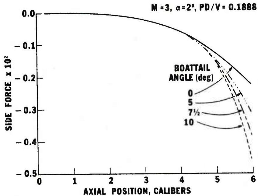
Figure 12. Magnus Force Coefficient versus Axial Position, Parametric Comparison, M = 3 , \alpha = 2^\circ , PD/V = .19 , T_w = T_{aw} , Re = 6.80 \times 10^7/m
