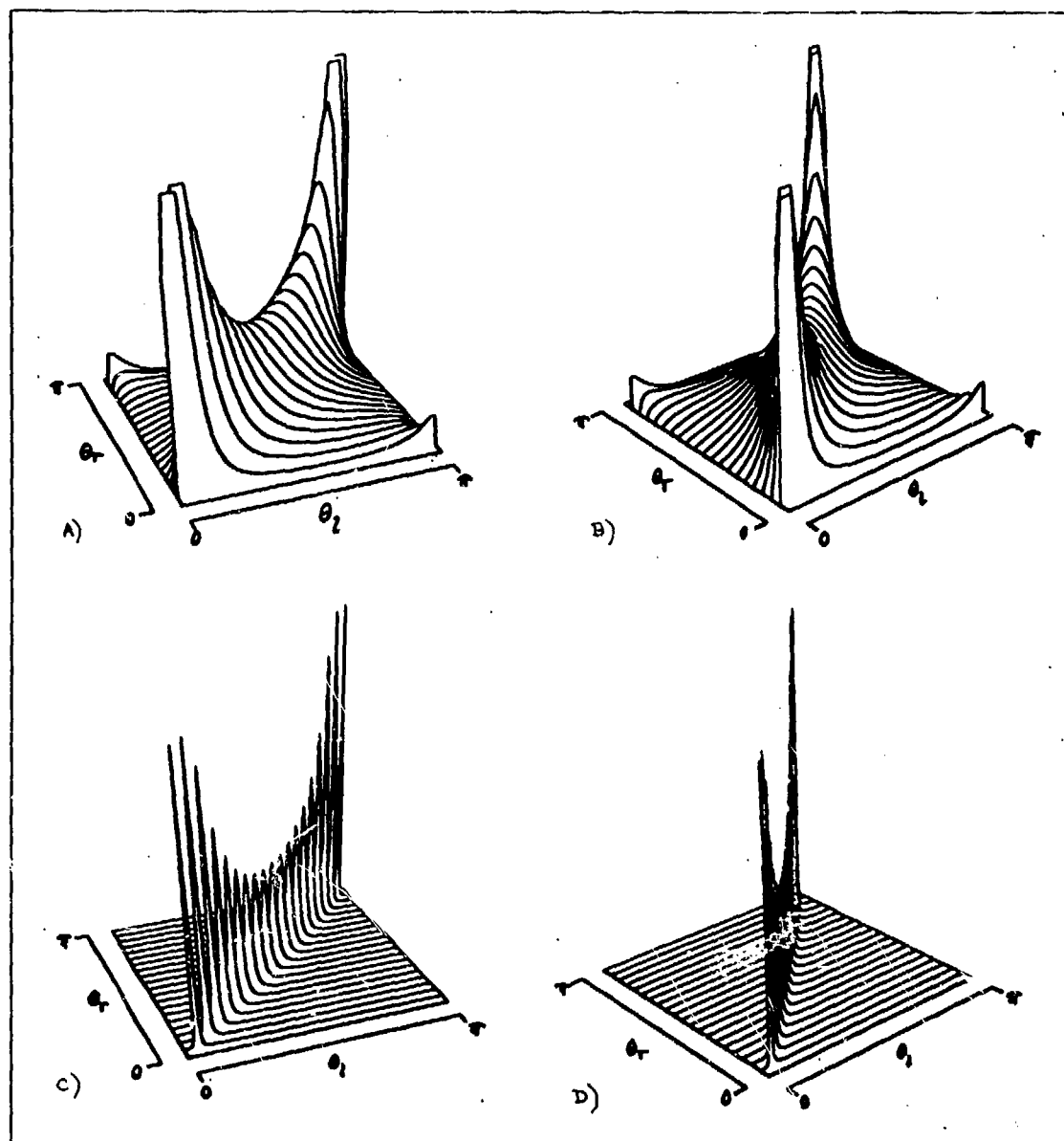
Figure 2-14: Probability density is plotted against image angles to show which combinations of angles are most likely to occur. The curves peak near the line \theta_l = \theta_r , indicating that the angles in the two images are most likely to be very similar. The shape of the curves varies with the camera geometry. Graphs a and b are two views of the function for a wide baseline ( B/z = .7 ). Graphs c and d show the much sharper function for a narrow baseline ( B/z = .07 ).
