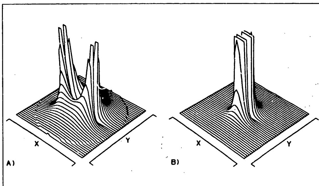
Figure 3-15: If edges from the left and right images were matched at random, the 3-dimensional orientations of the reconstructed scene edges would be distinctly non-uniform. A uniform distribution of image edge angles maps to a distribution on the gaussian sphere that is strongly peaked along the line of sight of the two cameras. Surfaces a and b result from baselines of B/z = .7 and B/z = .07 , respectively.
