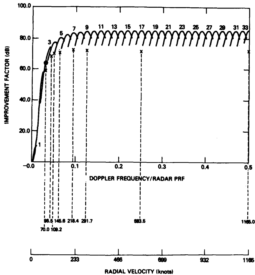
Fig. 18 — Modeled target (Xs) superimposed on the improvement factor curves. The horizontal pointing angles are 0^\circ (targets) and 90^\circ (filter design). The clutter-to-noise ratios are 55 dB (targets) and 65 dB (filter design).
