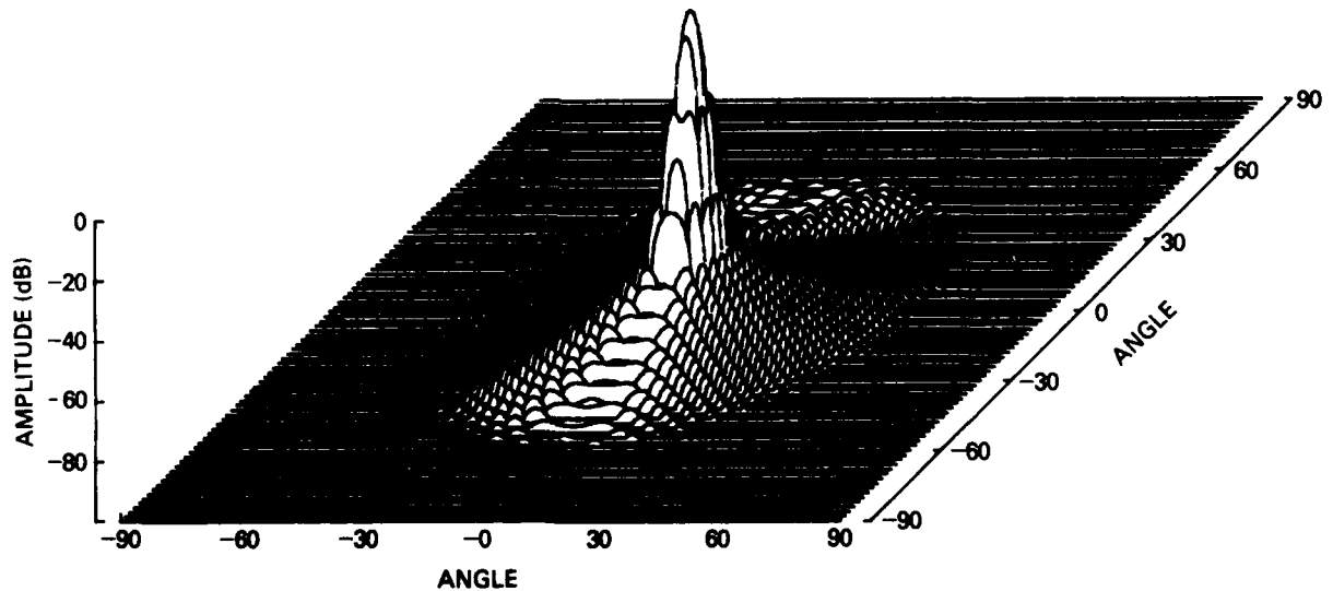
Fig. A3 — Two-way circular antenna pattern with a 1.5-m aperture, uniform weights on transmit, 34-dB truncated Gaussian weights on receive, and frequency of 3 GHz
