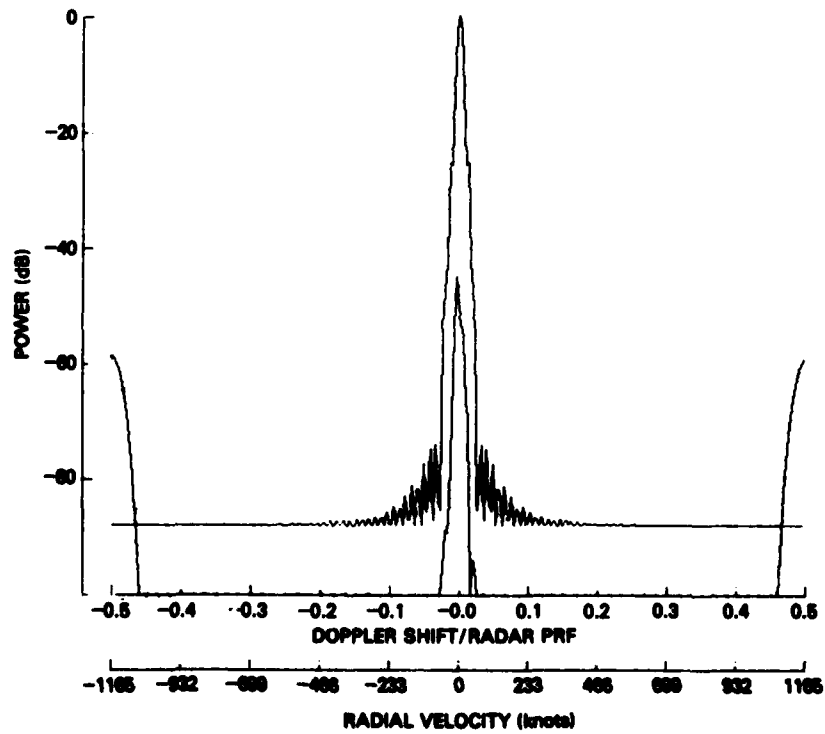
Fig. 14 — Input and output spectra of filter No. 33
