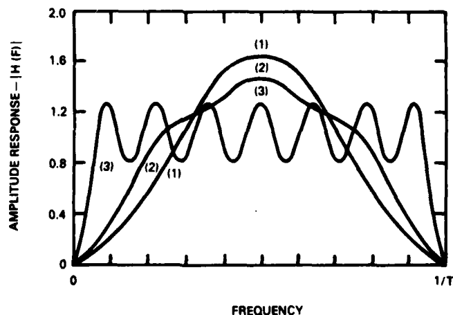
Fig. 11 — Amplitude responses for three MTI delay-line cancellers. (1) Classical 3-pulse canceller, (2) 5-pulse delay-line canceller with "optimum" weights, and (3) 15-pulse Chebyshev design. (After Houts and Burlage [9].)
