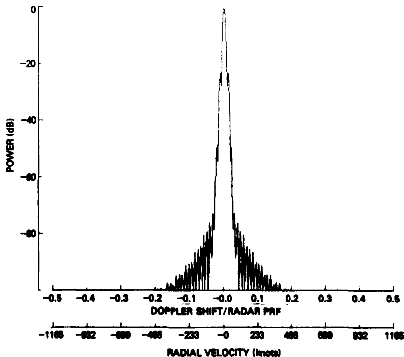
Fig. 2 - Clutter spectrum due to platform motion; 5 nmi (30 000 ft) altitude, 50-kHz pulse repetition frequency, azimuth is 90^\circ
