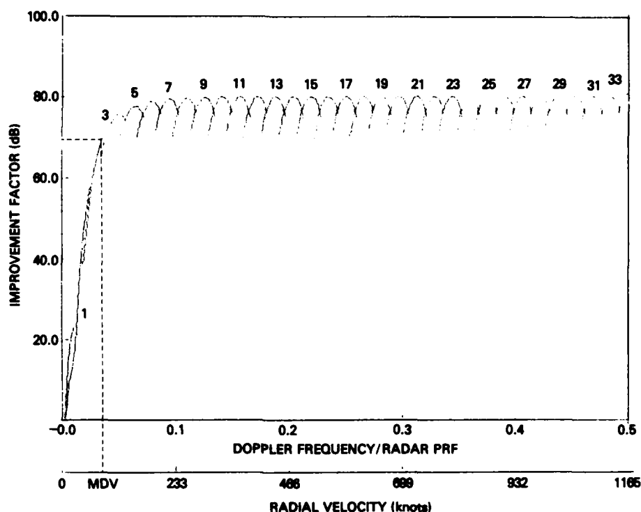
Fig. 6 — Improvement factor for a 64-pulse Doppler processor using the matched filter algorithm preceded by a single-canceller MTI. The clutter-to-noise ratio is 65 dB.
