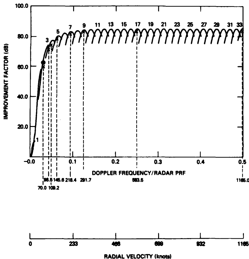
Fig. 16 — Matched filter modeled target outputs (Xs) superimposed on the matched filter improvement factor curves. The horizontal pointing angle is 90^\circ (for both targets and filter design). The clutter-to-noise ratio is 65 dB (for both targets and filter design).
