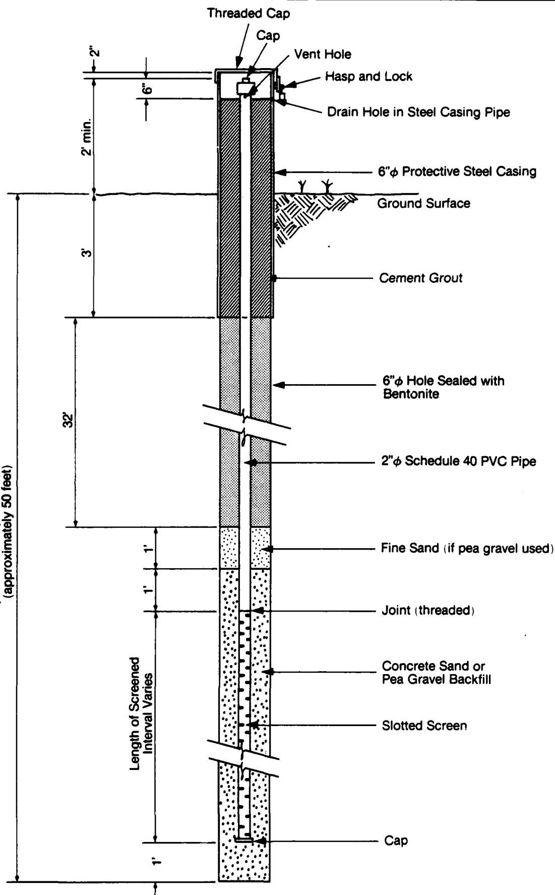
FIGURE 25. Typical Monitoring Well Installation.
