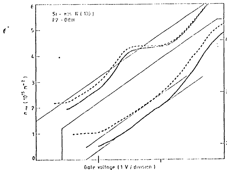
Figure 6. Gate voltage dependence of inversion layer carrier density, n_{inv} , for two different substrate bias conditions: --- V_{sub} = 0 ; - - - V_{sub} = 5 V, B = 9 T; T = 1.2 K. The plateau is observed when V_{sub} = 5 V. The straight line is the carrier concentration obtained from n_{inv} = C_0(V_g - V_1)/e , where the threshold voltage V_1 was determined from the period of the Shubnikov-de Haas oscillation in the standard way.
