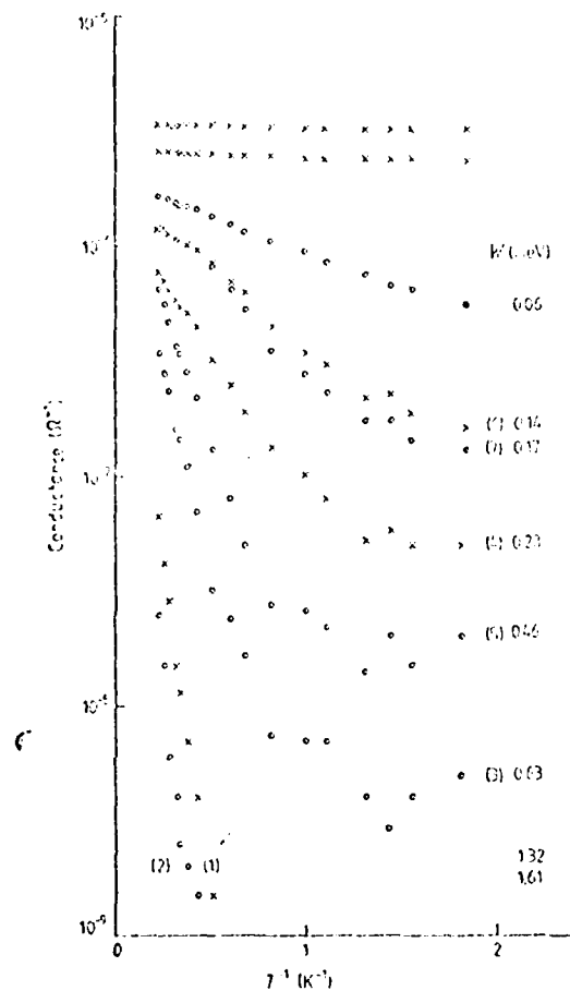
Figure 5. Detailed temperature dependence of conductance of the structure shown in figure 4; the location of the Fermi energy is indicated by the numbers (1, 2, . . . 7) in figure 4, V_{SD} = 0.1 mV. The activation energies are indicated for the maxima 1, 4, 6 and minima 2, 3, 5 and 7. Crosses denote maxima; circles denote minima.
