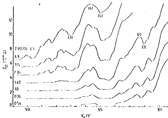
Figure 4. The temperature dependence of the oscillations in a structure subjected to avalanching. V_{DS} was 0.1 mV. The numbers indicate the location of E_1 used in figure 5.
