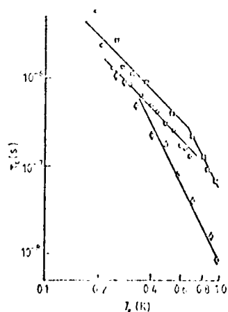
Figure 4. Energy relaxation time versus electron temperature for different values of the elastic mean free path l_e on log scales. The lines drawn show \tau_e \propto T_e^{-1} , \tau_e \propto T_e^{-2} .
