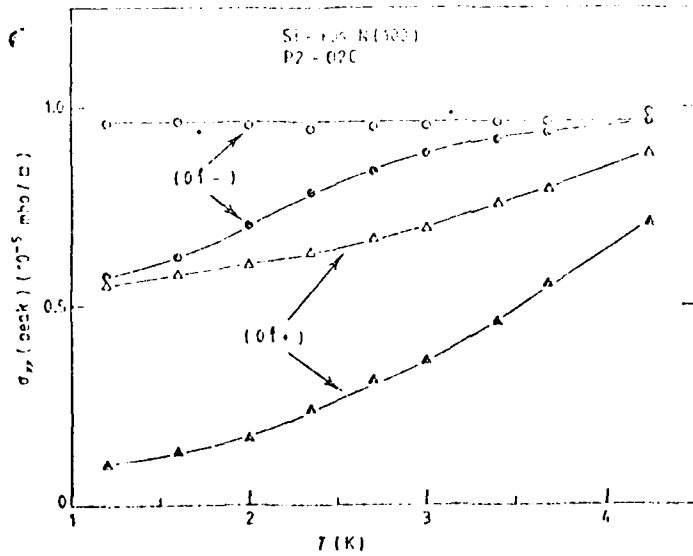
Figure 2. Temperature dependence of peak values of \sigma_{xx} of (0 \uparrow -) and (0 \uparrow +) levels at two different values of source-drain field. Full symbols, E_{SD} = 0.0 \text{ V cm}^{-1} ; open symbols, E_{SD} = 4.0 \text{ V cm}^{-1} ; B = 9 \text{ T} .
