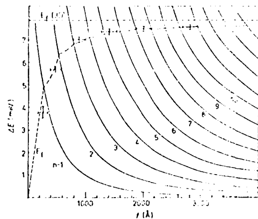
Fig. 1: Experimental and theoretical variation of E_F with t for N_D = 5.5 \cdot 10^{17} \text{ cm}^{-3} ( \epsilon = 1.38 ). The subband energies \Delta E_n for n = 1, 2, 3 \dots are referenced to the groundstate subband energy at n = 0 .
