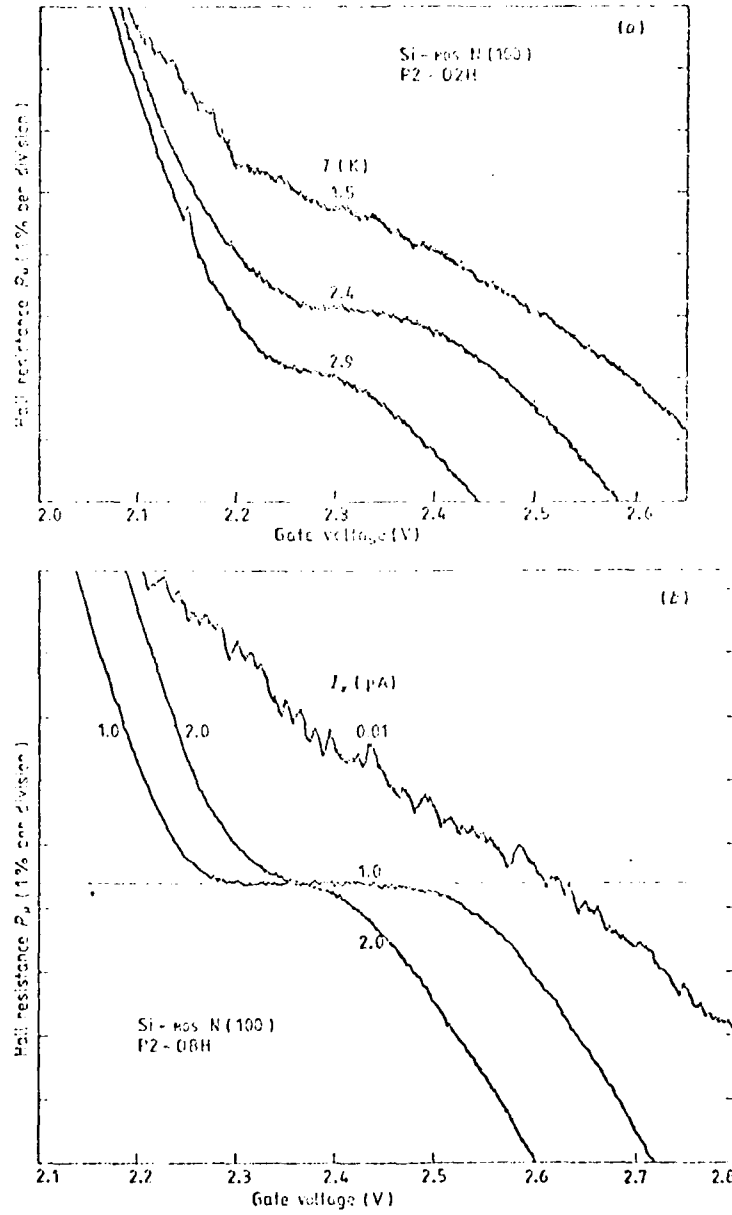
Figure 4. (a) Temperature dependence of plateau region between (0 \uparrow \downarrow) and (0 \downarrow \uparrow) levels ( I_s = 0.05 \mu\text{A} ); (b) Current dependence of plateau region between (0 \uparrow \downarrow) and (0 \downarrow \uparrow) levels ( T = 1.2 \text{ K} , H = 9.0 \text{ T} ; f = 180 \text{ Hz} ).
