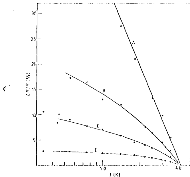
Figure 5. The percentage change in R , \Delta R/R , is plotted against T normalised to T = 4.2 K for various values of E_1 . The full curves are for a guide only. A, E_1 = 83 meV; B, 173 meV; C, 207 meV; D, 305 meV.
