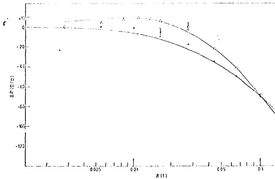
Figure 2. \Delta R is plotted against B for T = 4.2 K (G) and T = 1.25 K (Z). T_{1/2} = 5.0 mV corresponding to kT = 8 . The full curves are the theoretical calculations from equation (6) with \tau_0 = 4.5 \times 10^{-12} .
