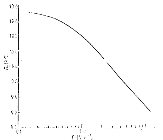
Figure 3. Variation of differential resistivity with electric field. The curve is obtained by numerically integrating figure 2.
