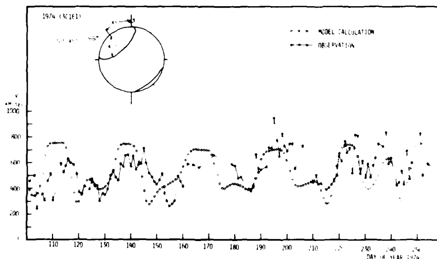
Figure 4. Observed and calculated IPS pattern speeds and the model calculations (using an 800 km/sec tilted polar high-speed source region) for 1974. The IPS source is 3C161 (UCDS observations).
