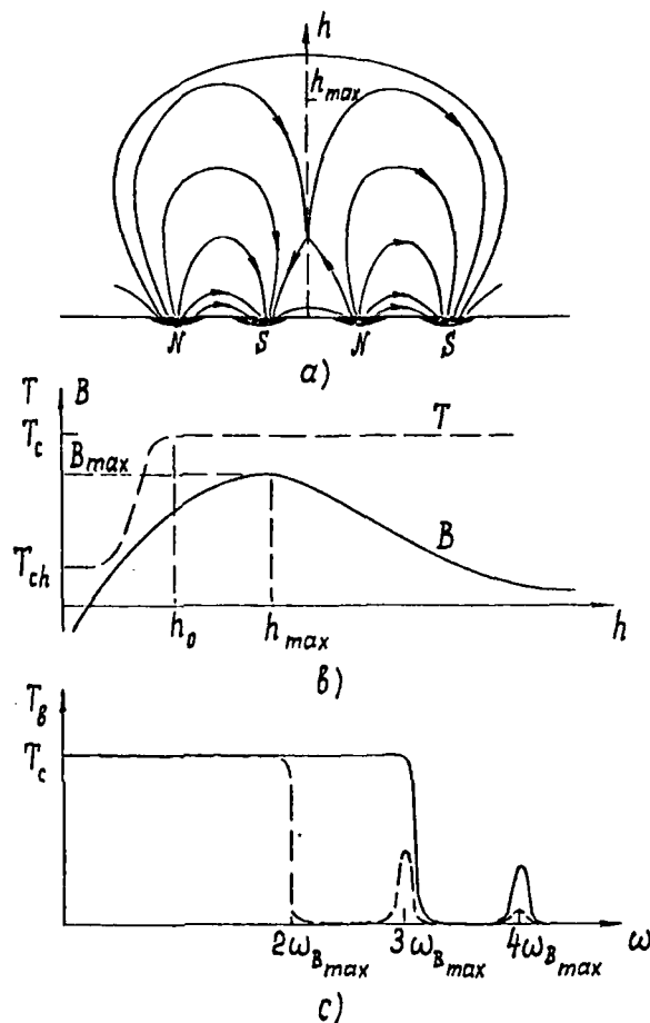
Figure 2. The model of a source with the maximum of the magnetic field over height: a) magnetic lines of force above a group of sunspots ( h_{\max} is the height at which the magnetic field has its maximum value); b) distribution of the magnetic field and kinetic temperature over the height; c) the frequency spectrum of radiation.
